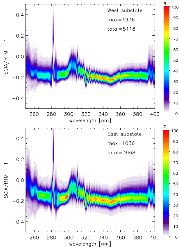
Fig. 2. Spectra of histograms of the relative difference between measured and calculated reflectances, normalised to the maximum value. (top) For West substates; (bottom) for East substates. In total, 3968 valid East substates are included, and 5118 valid West substates. The peak near 282 nm is a Fraunhofer line which has not been masked out in our analysis. The feature near 305 nm is due to the ozone profile used as input for the RTM.
