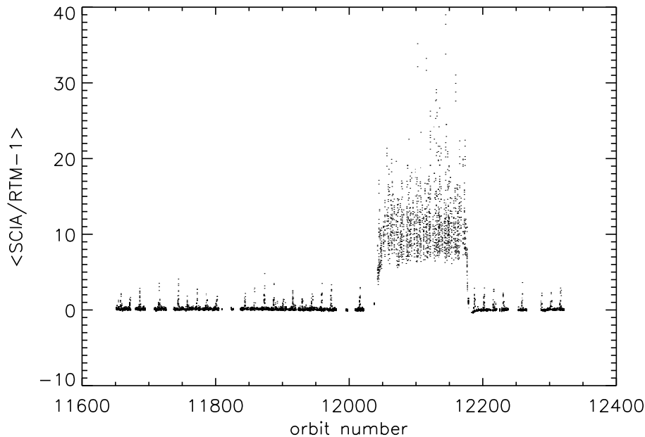
Fig. 7. Time series of \bar{d}_R(280) showing the effect of decontamination, between orbits 12031 and 12208 (18–30 June 2004), on channel 1. d_R rises to a value around 10 (1000%)! The usual assumption is that the UV-Vis channels of SCIAMACHY are not affected by decontaminations. The periodic small peaks rising to about 2 during the rest of the period are caused by states in the SAA.
