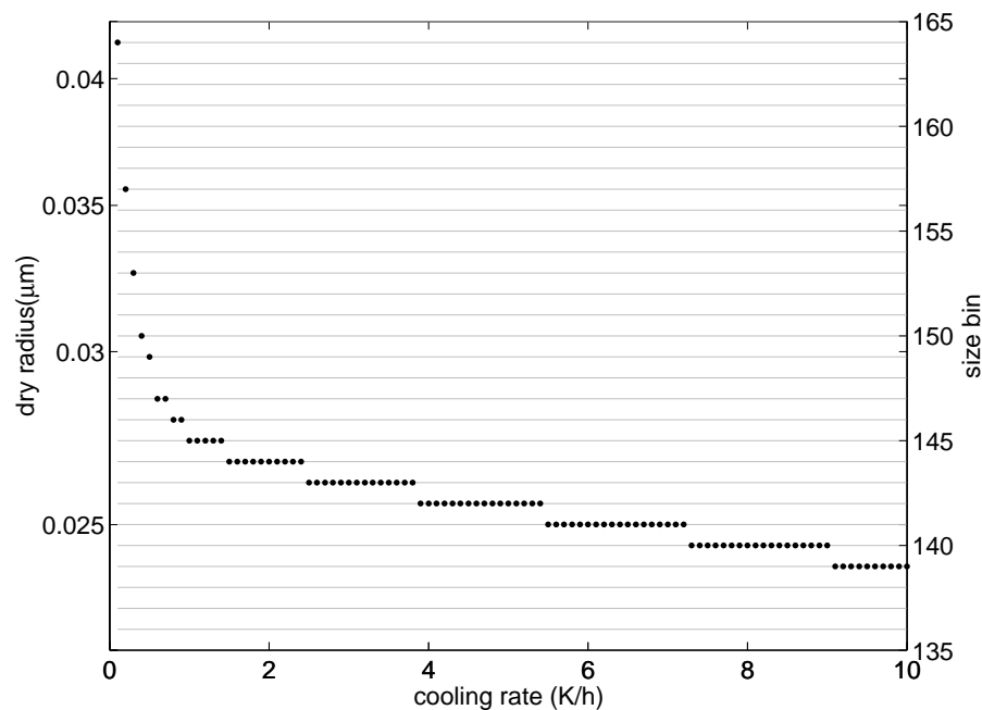
Fig. 5. The size bin under which a gap in the size distribution appears calculated and the corresponding dry radius of the particles in the size bin as a function of cooling rate.
