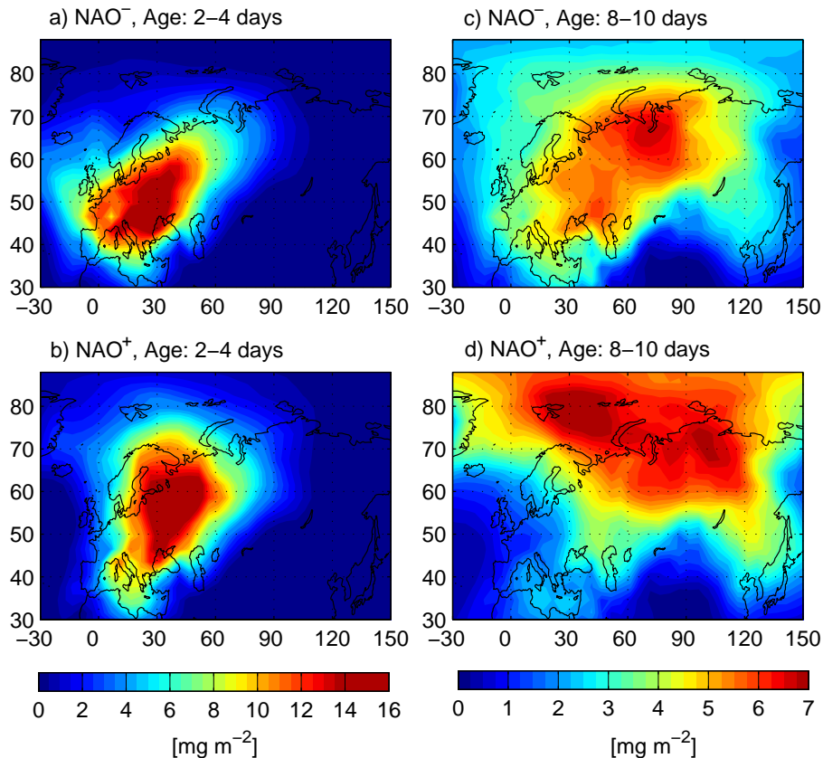
Fig. 2. European tracer columns [ \text{mg m}^{-2} ] 2–4 days (a, b), and 8–10 days (c, d) after tracer emission. The two composites represent the three December, January and February months with the lowest and highest NAO index, respectively, selected from a 15-year (1979–1993) period.
