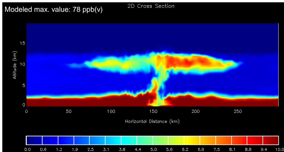
Fig. 5. (h) Modeled SO 2 concentration (ppbv) after 3 h simulation. The modeled value at 10.4 km is indicated in the figure.
