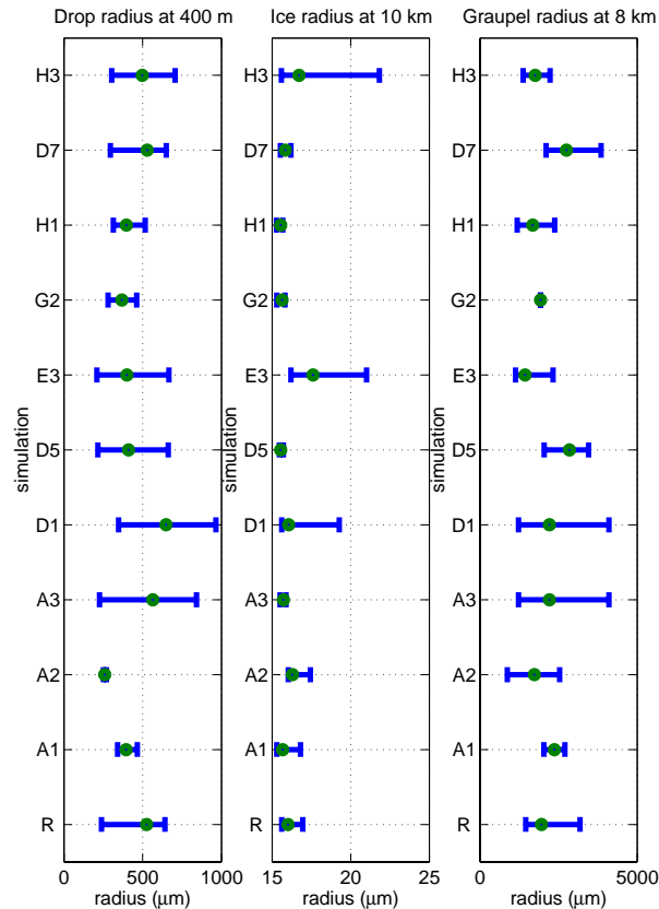
Fig. 11. (b) Average (both horizontally and over 3 h of simulation) effective rain droplet radius, ice particle radius and graupel radius at 400 m, 10 km and 8 km, respectively. Also shown in the figure are the maximum and minimum horizontally averaged effective radii simulated over the 3 h period.
