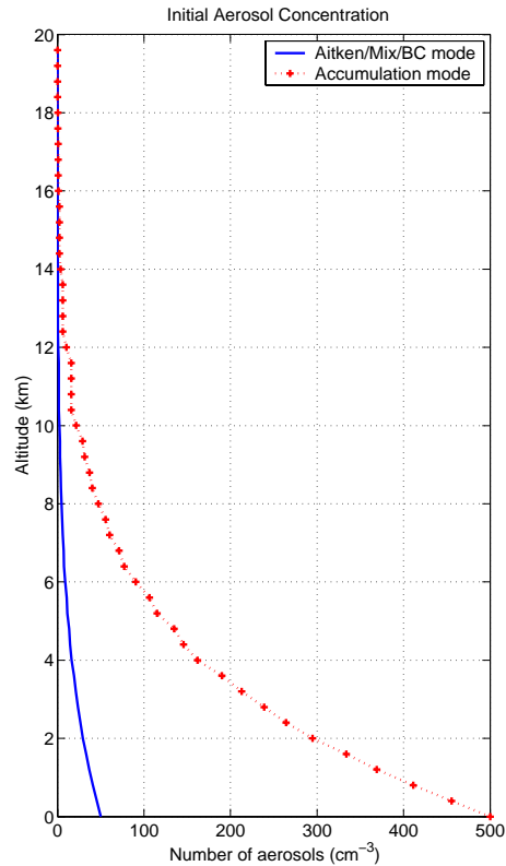
Fig. 2. Vertical profile of initial aerosol concentration.
