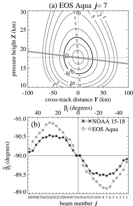
Fig. 11. (a) W_j(Y, Z) at j=7 for AMSU-A on EOS Aqua. Contours are power values relative to the peak value expressed as a percentage. The 50% contour is shown in bold. Dotted gray line shows the line-of-sight ray to the satellite. Solid gray curve connects local maxima in vertical cross sections through the weighting function at different Y , and specifies the cross-track tilt axis Y'_j . The off-nadir tilt angle of this gray line is \tilde{\beta}_j . (b) \tilde{\beta}_j angles computed as in (a) for all the weighting functions W_j(Y, Z) for both the NOAA (solid curve) and EOS Aqua (dotted curve) AMSU-A.
