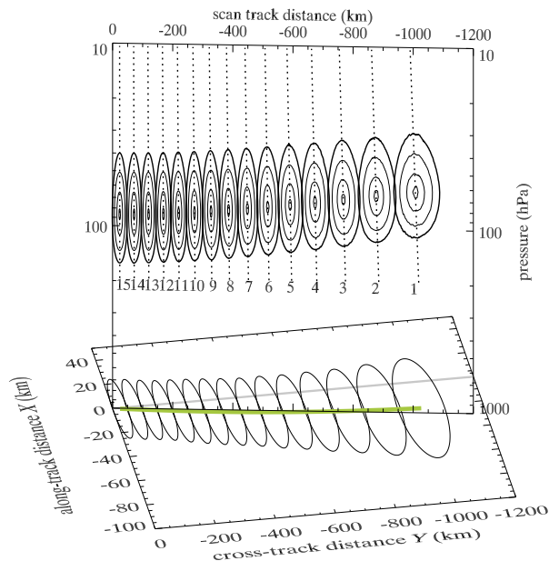
Fig. 4. Modeled AMSU-A Channel 9 weighting functions W_j(Y, Z) for beam positions j=1 \dots 15 . Thick contours show the half-power (50%) levels, the outer ranges of which are projected to the surface to depict the horizontal footprints. Other contours show the 70%, 90% and 99% levels. Dotted lines show line of sight ray paths from the peaks in each weighting function to the satellite point, taking into account Earth curvature: the off nadir angles \beta_j that each of these ray paths makes at the weighting function peak are plotted as the dotted curve in Fig. 2. The W_j(Y, Z) contours are plotted along a vertical plane aligned along an approximate scan axis that is offset slightly from the cross-track axis Y due to the 7.4 \text{ km s}^{-1} motion of the satellite along the X axis during the 3 s taken to scan through beam positions j=1-15 . The actual X - Y scan track is plotted in green, and curves slightly in the X - Y plane. Note the different X and Y axis scales: footprint diameters along track are in fact narrower than those cross track (see Fig. 5).
