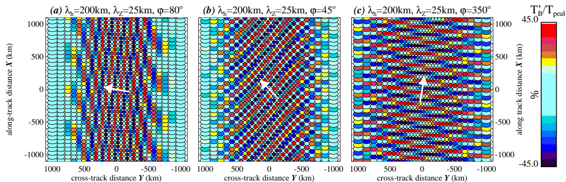
Fig. 14. Same presentation as in Fig. 13, but for a gravity wave with \lambda_{\parallel}=200 km, \lambda_{\perp}=25 km.
