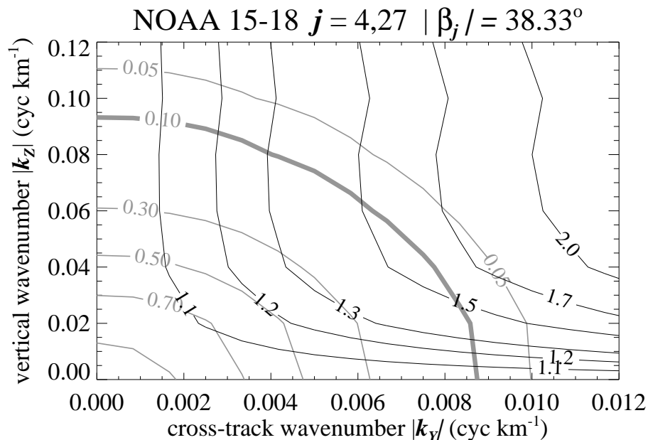
Fig. 15. Black contours show the spectral variance visibility ratio \hat{R}_{j,j}^2(k_Y, k_Z) as a function of cross-track and vertical wavenumber for the NOAA AMSU-A j=4, j_*=27 conjugate beam pairing. Gray lines overlay absolute visibility contours of \hat{W}_j(k_Y, k_Z) for the j=4 beam.
