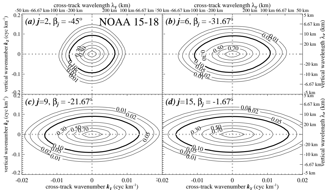
Fig. 8. Fourier Transforms \hat{W}_j(k_Y, k_Z) computed from the model-generated 2-D Channel 9 weighting functions W_j(Y, Z) in Fig. 4 and normalized to a peak response of unity, for (a) j=2 ( \beta_2=-45^\circ ), (b) j=6 ( \beta_6=-31.67^\circ ), (c) j=9 ( \beta_9=-21.67^\circ ), and (d) j=15 ( \beta_{15}=-1.67^\circ ).
