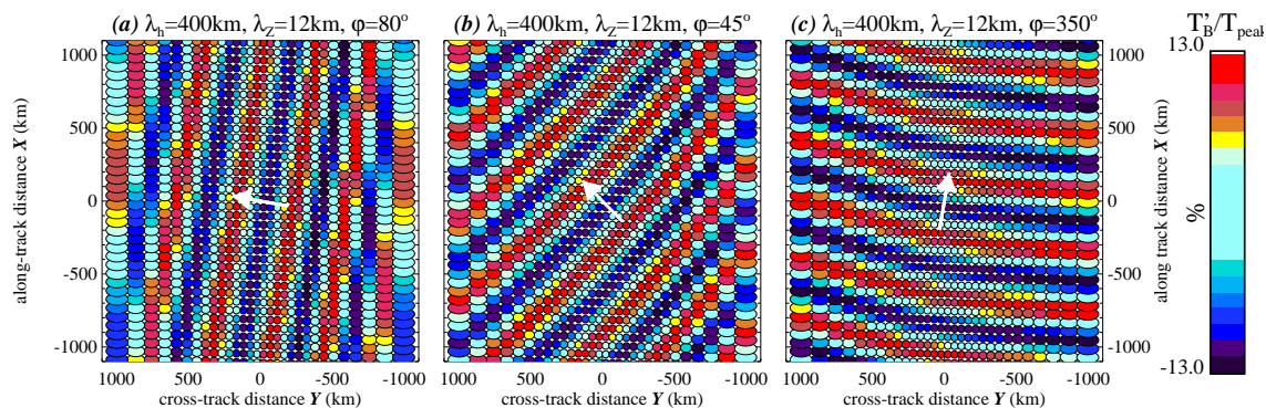
Fig. 13. (a) Relative brightness temperature perturbations (visibilities) T'_B(X_j, Y_j)/T_{\text{peak}} resulting from model NOAA AMSU-A Channel 9 sampling of a gravity wave in Eq. (15) with T_{\text{peak}}=5 K, \lambda_n=400 km, \lambda_z=12 km, and \varphi values of (a) 80^\circ , (b) 45^\circ , and (c) 350^\circ . The white vector at the center of each plot shows this direction of horizontal wave propagation \varphi . The color scale is the visibility amplitude expressed as a percentage, indicating a peak sensitivity of \sim 13\% , or a maximum brightness temperature perturbation of \sim 0.65 K.
