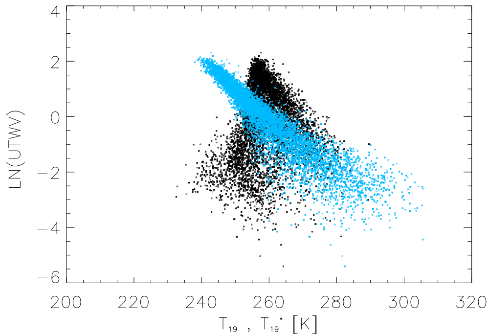
Fig. 7. As Fig. 6 but for AMSU-B channel 19.
