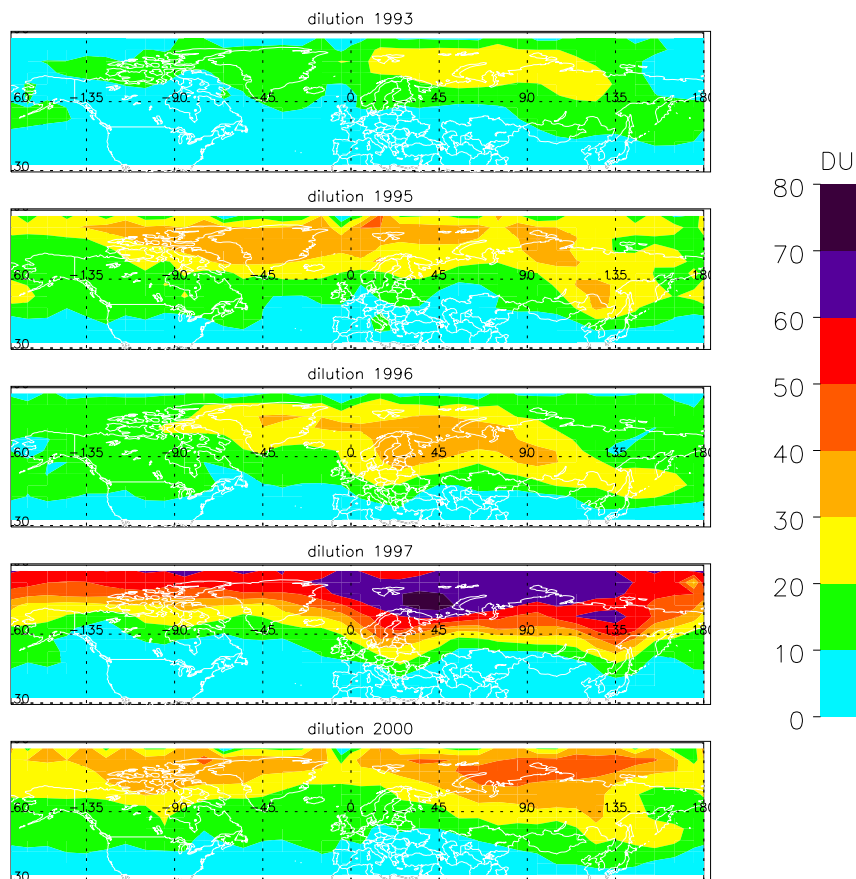
Fig. 1. April–May averages of the ozone depletion originating from the polar vortex in 1993, 1995, 1996, 1997, and 2000. 5° latitude-longitude boxes were used. In 1997 the total depletion was largest and the vortex broke up latest, so that the mixing to lower latitudes was weakest.
