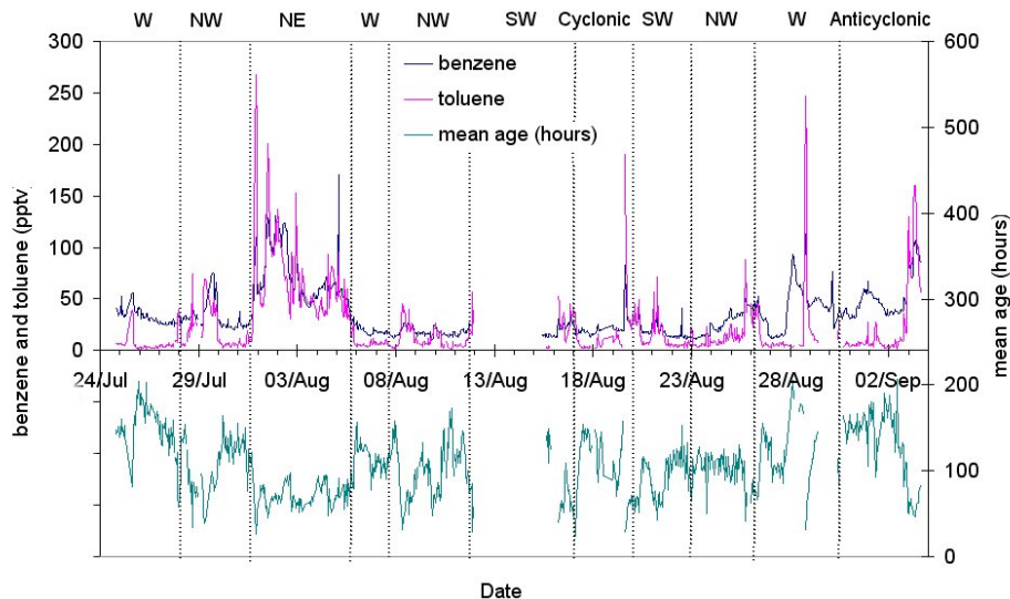
Fig. 2. Benzene and toluene observations versus Julian day 2002, used as markers for airmass pollution ‘age’ arriving at the site. (Assumes a starting ratio of 1:4.4 and [\text{OH}] = 1 \times 10^6 \text{ molecules cm}^{-3} , rate constants from Atkinson, 1986, 1989). Time series subdivided into periods with distinct airmass origins. Data with contradictory local wind direction/trajectory origin/chemical signatures were subsequently excluded from airmass type average calculations.
