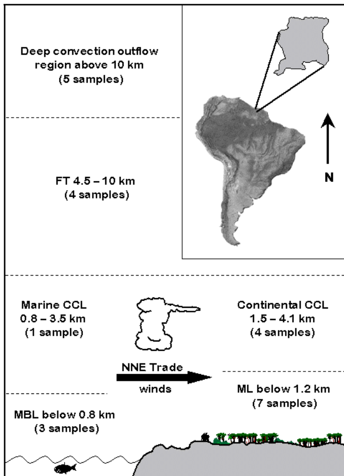
Fig. 1. Schematic picture of the stratification of the samples into the distinct atmospheric layers present in the tropical troposphere over Surinam and the adjacent coastal Atlantic Ocean. The number in parentheses indicates the number of samples analyzed in each layer.
