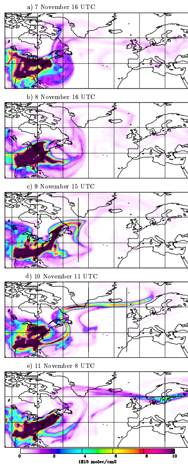
Fig. 6. Total vertical columns of the FLEXPART \text{NO}_x tracer (in 10^{15} molecules \text{cm}^{-2} ) on (a) 7, (b) 8, (c) 9, (d) 10, and (e) 11 November. The columns are averages over 1-h periods ending at 16, 16, 15, 11, and 08:00 UTC, respectively. Bold black lines mark meridional sections shown in Fig. 7.
