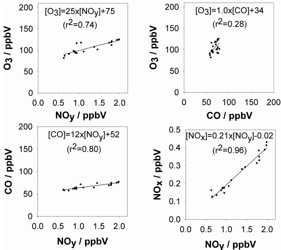
Fig. 10. Trace gas correlations for the plume between 9 and 10 km altitude of MINOS flight 9 (17 August 2001), see Fig. 9. All plots show high correlations except for \Delta[O_3]/\Delta[CO] . The uncertainties of the slopes and the intercepts are given in Table 3 and in the text, respectively.
