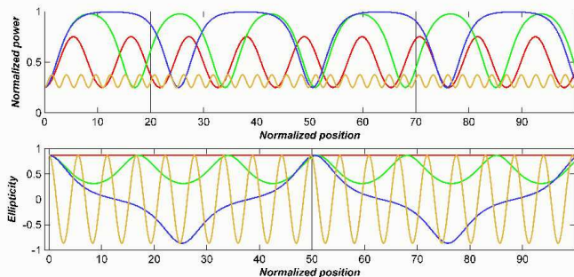
Fig. 9. Evolution of power in the x-axis and ellipticity versus normalized fiber position for different polarization states at the fiber input (no fiber attenuation, with birefringence).
