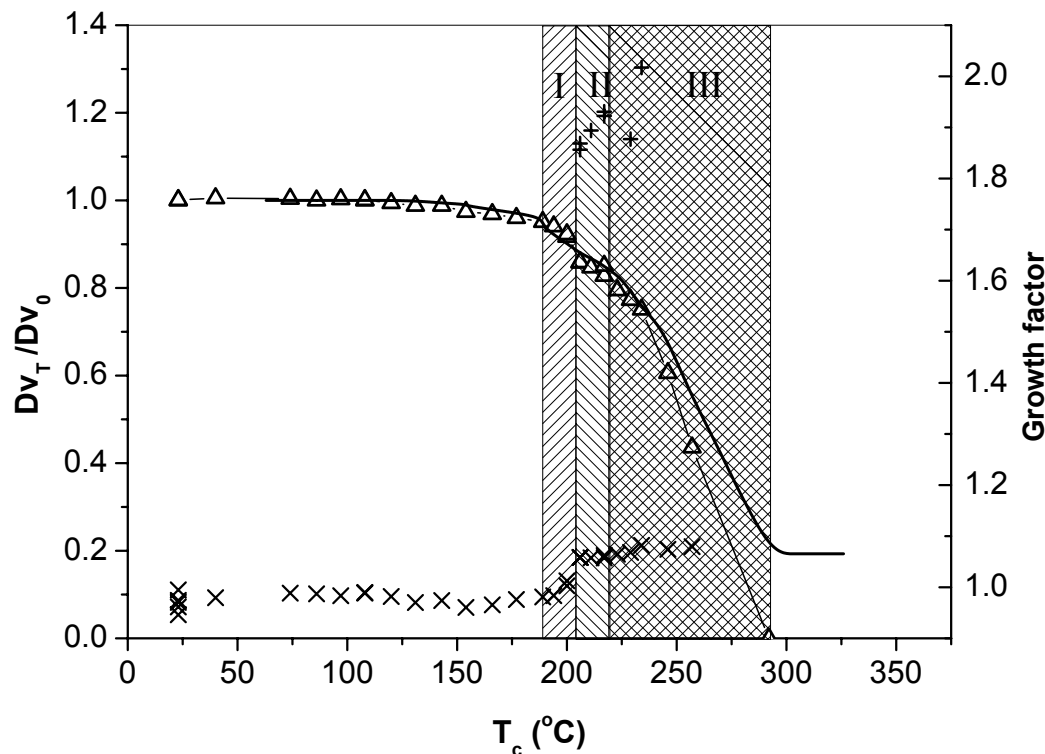
Fig. 4. VH-TDMA spectra of 80 nm photochemically produced aerosols, showing the relative diameter after volatilisation D_{v_T}/D_{v_0} – triangles; and the hygroscopic growth factors G = D_h/D_v versus thermodenuder temperature, for both hygroscopic G_h (+) and non-hygroscopic G_{nh} (x) peaks. The sheath gas was filtered air. The volatility curve of \text{HIO}_3 particles of similar size measured in air as sheath gas is also shown with a full line.
