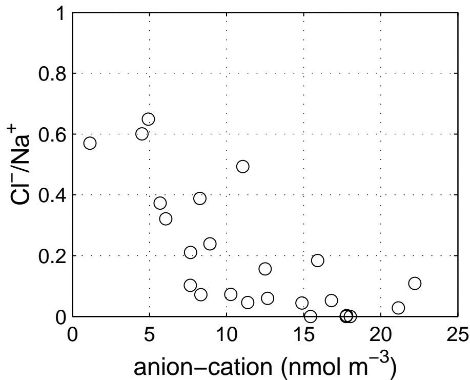
Fig. 8. The fpm \text{Cl}^-/\text{Na}^+ molar ratio as a function of the difference between the analysed cations and anions (referred to as acidity) for samples in the IInd and sIInd trajectory groups during the Ronald H. Brown cruise in 1999.
