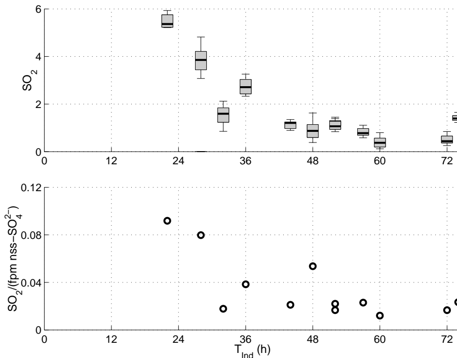
Fig. 7. (a) The SO 2 concentration as medians over the aerosol sampling time (~6 h) as a function of transport time from India during the Ronald H. Brown cruise in 1999. The box includes data between the 25 and 75 percentiles and the vertical bars represent the 10 and 90 percentiles. (b) The SO 2 /(fpm nss-SO 4 2- ) molar ratio, as a function of transport time from India during the Ronald H. Brown cruise in 1999.
