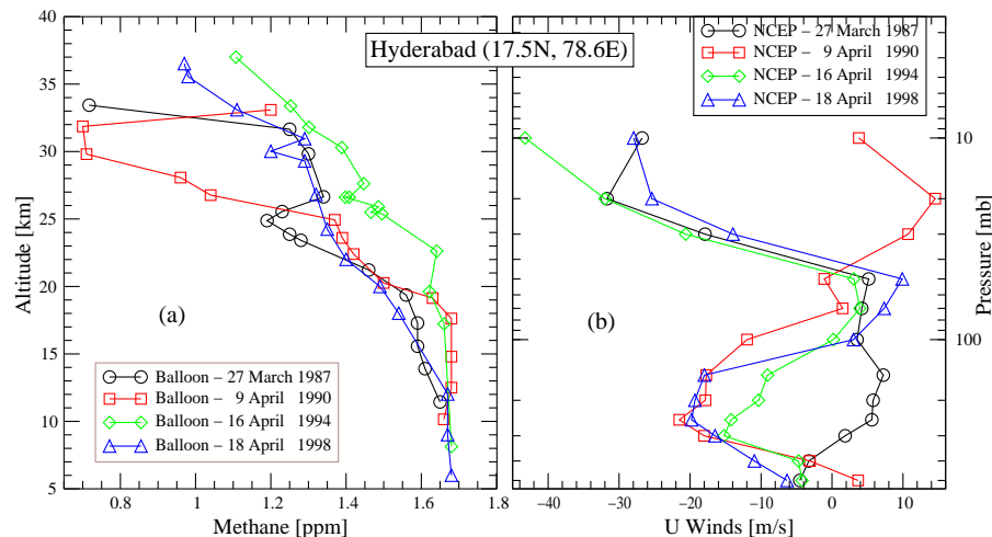
Fig. 1. Vertical profiles of CH 4 obtained by analyzing the ambient air collected during the cryo-sampler experiments in boreal spring of 1987, 1990, 1994 and 1998. The 1987 and 1990 profiles are obtained from the PRL-MPAE collaborative programme (Borchers et al., 1989), and 1994 and 1998 profiles are from the PRL conducted experiments (Lal et al., 1996).
