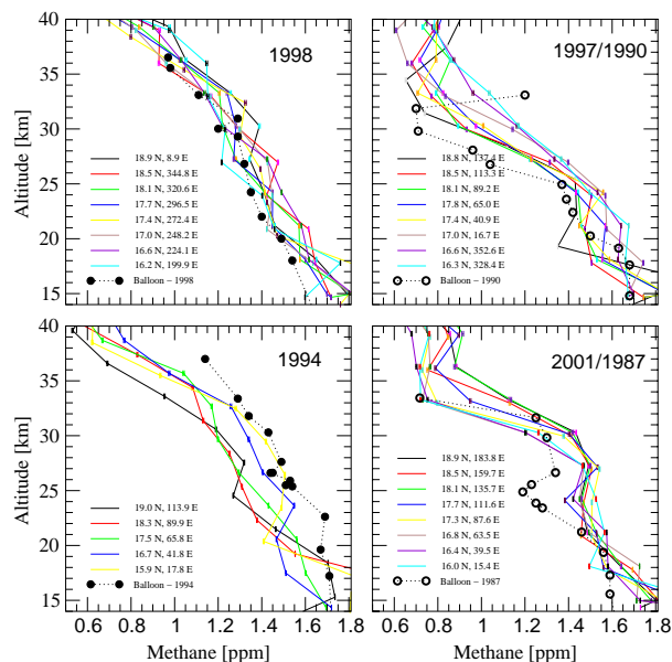
Fig. 4. Showing the match between the remote sensing observations with in situ measurement of CH 4 . The comparison of 1994 and 1998 balloon measurements (filled circle) with the HALOE CH 4 profiles are shown as they were observed in the respective years (panels on the left). Whereas for 1987 and 1990 balloon data (open circle), we have chosen the HALOE profiles from the years 2001 and 1997, respectively, for comparison (right panels) due to the lack of contemporaneous HALOE measurements, which are selected based on the meteorology of the stratosphere. The time and type of all HALOE measurements can be designated as: 1) 5 April (22:17 GMT) to 6 April (04:43 GMT) in 1994 (Sunrise), 2) 12 April (17:36 GMT) to 13 April 04:50 GMT) in 1998 (Sunset), 3) 17 April (09:03–20:17 GMT) in 1997 (Sunset), and 4) 27 March (05:52–17:05 GMT) in 2001 (Sunset). The HALOE profiles are chosen as close to balloon measurement dates as possible irrespective of sunset or sunrise data retrieval.
