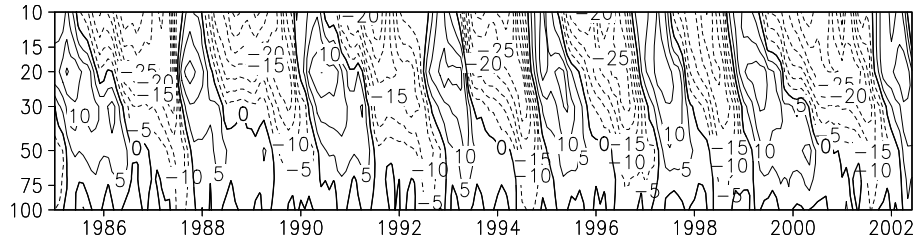
Fig. 3. Temporal variations in monthly mean zonal wind anomalies (m/s) with respect to pressure (mb), produced by the NCEP/NCAR reanalysis project over the equator. The contour interval is 5 m/s; negative wind speed represents the Easterlies (denoted by dotted lines), and the Westerly phase of QBO is seen as the positive winds (solid lines). Note that the height extent of QBO is approximately from 100 mb to 10 mb, and above 3 mb (not shown here due to the lack of NCEP/NCAR reanalysis data beyond 10 mb height) dominance of the semi-annual oscillation (SAO, westerly near the equinox and easterly near the solstice) over QBO is apparent (Swinbank and O'Neill, 1994).
