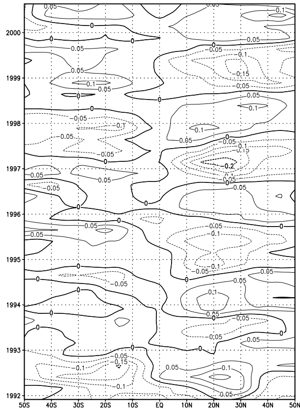
Fig. 6. Latitude-time crosssection of CH 4 anomaly showing the detailed latitudinal extent of QBO signal at 10 mb pressure layer. It can be noticed that the CH 4 anomalies in NH and SH are separated by a time lag of about one year.
