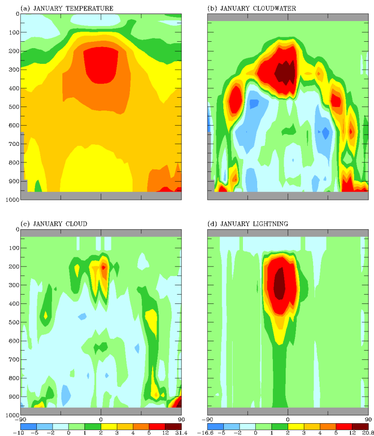
Fig. 3. (2100 ocean – control) in January (a) temperature (K), (b) cloudwater (ppmm), (c) total cloud cover (%) and (d) NO x from lightning ( 1 \times 10^{-2} kg/s).
