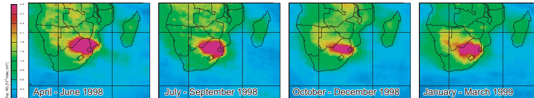
Fig. 2. Seasonal tropospheric NO 2 distribution of SA for 1998
