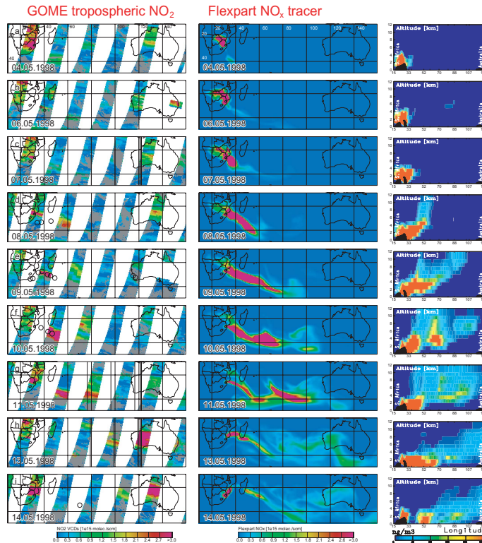
Fig. 3. Sequence of distributions of tropospheric \text{NO}_2 columns from the GOME instrument east of SA in May 1998 (left column). For the extraction of the tropospheric fraction of \text{NO}_2 the stratosphere/troposphere separation algorithm (Wenig, 2001) was used. Areas with high cloud cover (>50%) are masked in grey and areas with high lightning activity (> 50 flashes per grid cell) are marked by circles. Corresponding \text{NO}_x tracer column densities including emissions from lightning (centre column) and vertical sections of the \text{NO}_x tracer concentrations only for industrial emissions, averaged between 20 and 45 degrees southern latitude (right column), obtained with FLEXPART (see Appendix B).
