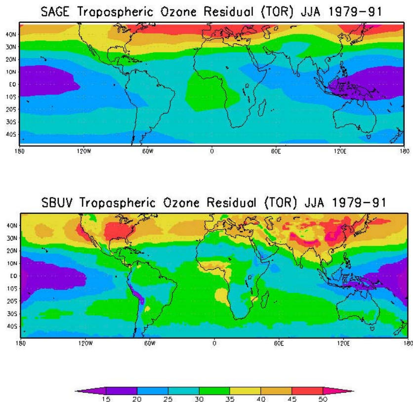
Fig. 2. TOR JJA distribution using the SAGE/TOMS technique described in Fishman and Brackett (1997) (top panel) and TOR calculated using the current technique. Both data sets use available measurements during the same period of time, 1979–1991.
