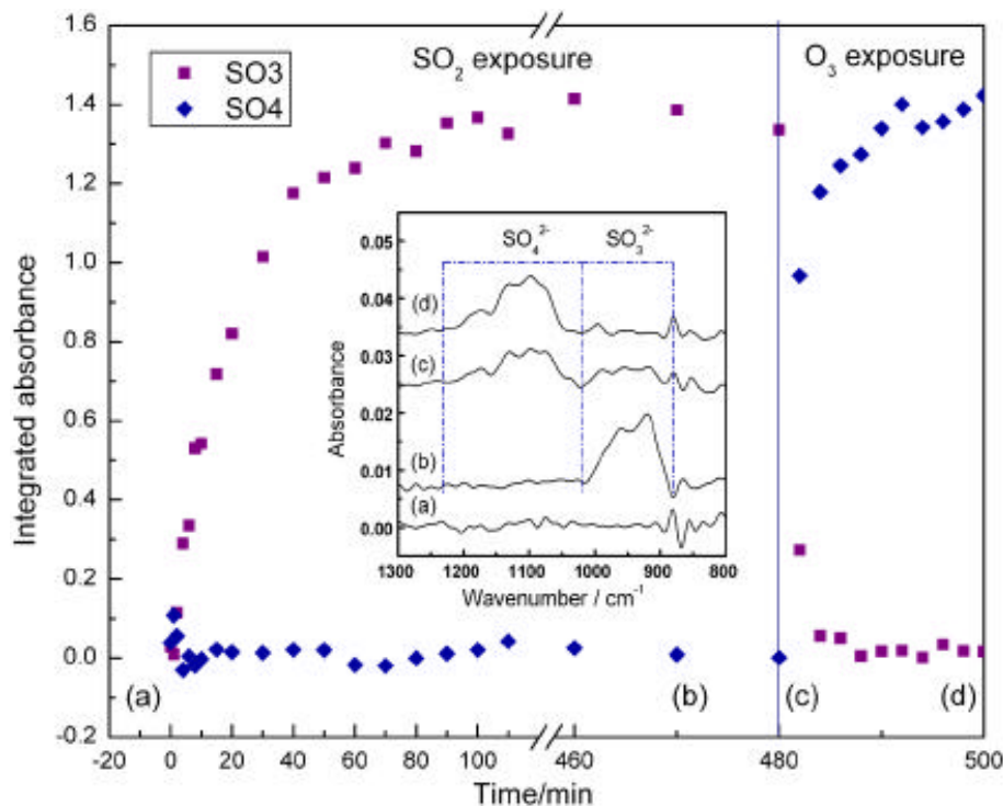
Fig. 2. Integrated absorbance of the DRIFTS band of sulfate and sulfite on CaCO 3 in the step-exposure experiment. The inset shows the in situ DRIFTS spectra recorded during the step-exposure experiment SO 2 and O 3 respectively. Product spectra (a) before addition of SO 2 , (b) the adsorption rate becomes stable after addition of SO 2 , (c) after cutting off SO 2 supply and the addition of O 3 for 4 min, (d) 30 min after the addition of O 3 . Spectra are shifted by +0.01, +0.025 and +0.035 absorption units, for (b), (c) and (d), respectively.
