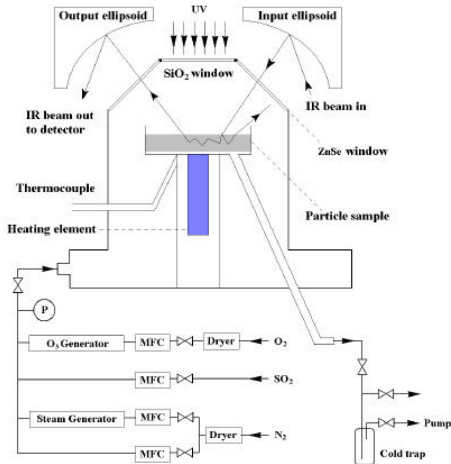
Fig. 1. Schematic diagram of the experimental set-up including the DRIFTS apparatus, the O 3 generator, steam generator, pressure gauge (P), mass flow controller (MFC), silicon and zeolite dryer, cold trap, pump and mixing lines.
