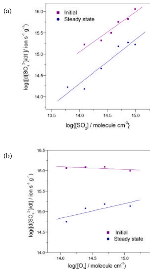
Fig. 8. Double-logarithmic plot of the rate of sulfate formation as a function of [\text{SO}_2] and [\text{O}_3] at initial time and steady state. The reaction order in \text{SO}_2 was determined from a linear regression yielding n_0=0.94\pm 0.06 ( \sigma ), n_{ss}=1.04\pm 0.13 ( \sigma ). For \text{O}_3 corresponding values are n_0=0.06\pm 0.26 ( \sigma ), n_{ss}=0.36\pm 0.45 ( \sigma ).
