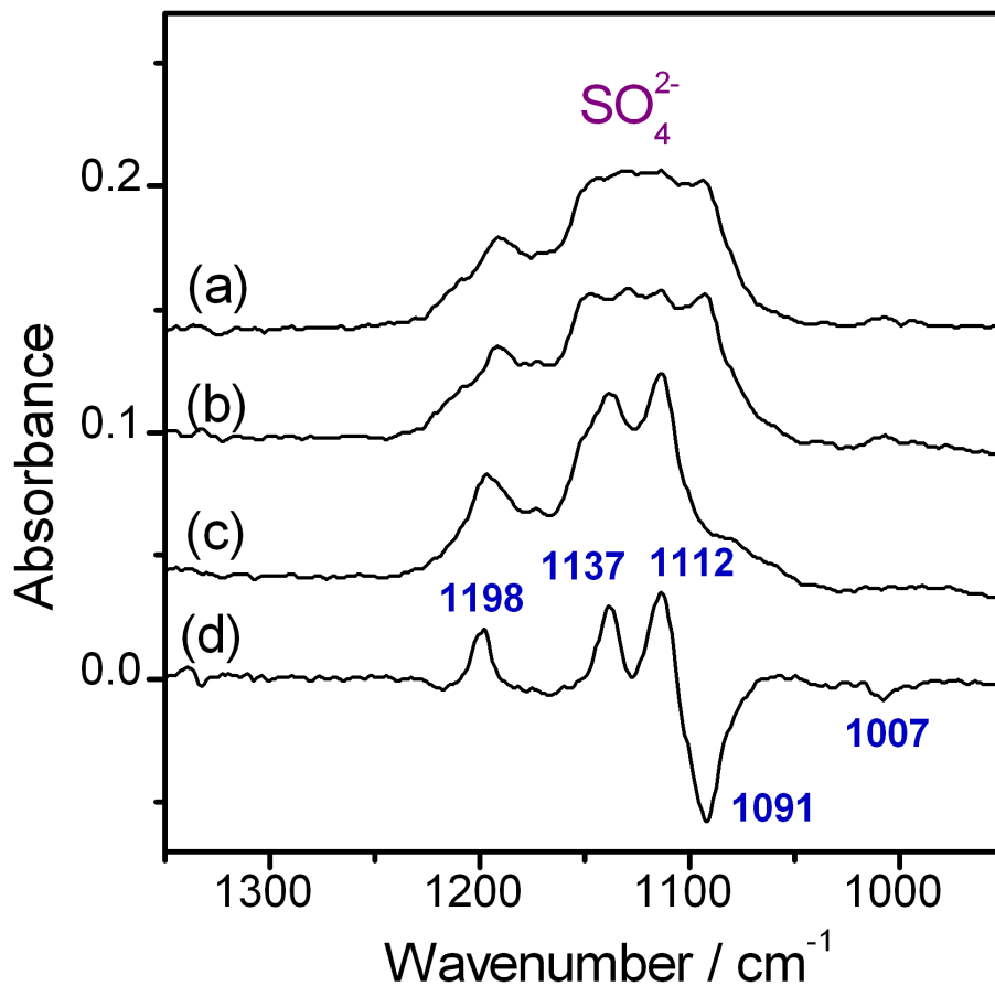
Fig. 5. Spectra of sulfate when the reactor with the sample was evacuated and heated. (a) Sample after a typical experiment with SO 2 and O 3 exposure, followed by evacuation to 10 Pa (b) and, further heating to 300°C (c) ; (d) difference between the spectrum (a) and (c).
