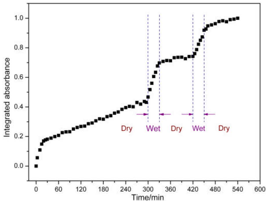
Fig. 9. Integrated absorbance of the sulfate band as a function of time in the reaction of \text{SO}_2 and \text{O}_3 on \text{CaCO}_3 . The vertical dashed lines indicate the time intervals when the sample was exposed to wet or dry air.
