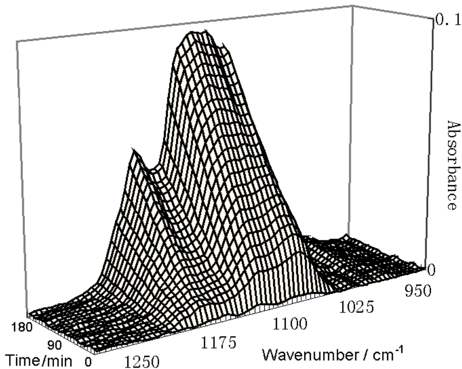
Fig. 4. Absorption bands observed during the reaction of SO 2 with O 3 on the surface of CaCO 3 as a function of reaction time ([SO 2 ]=4.92×10 14 molecules cm -3 , [O 3 ]=4.92×10 14 molecules cm -3 ).
