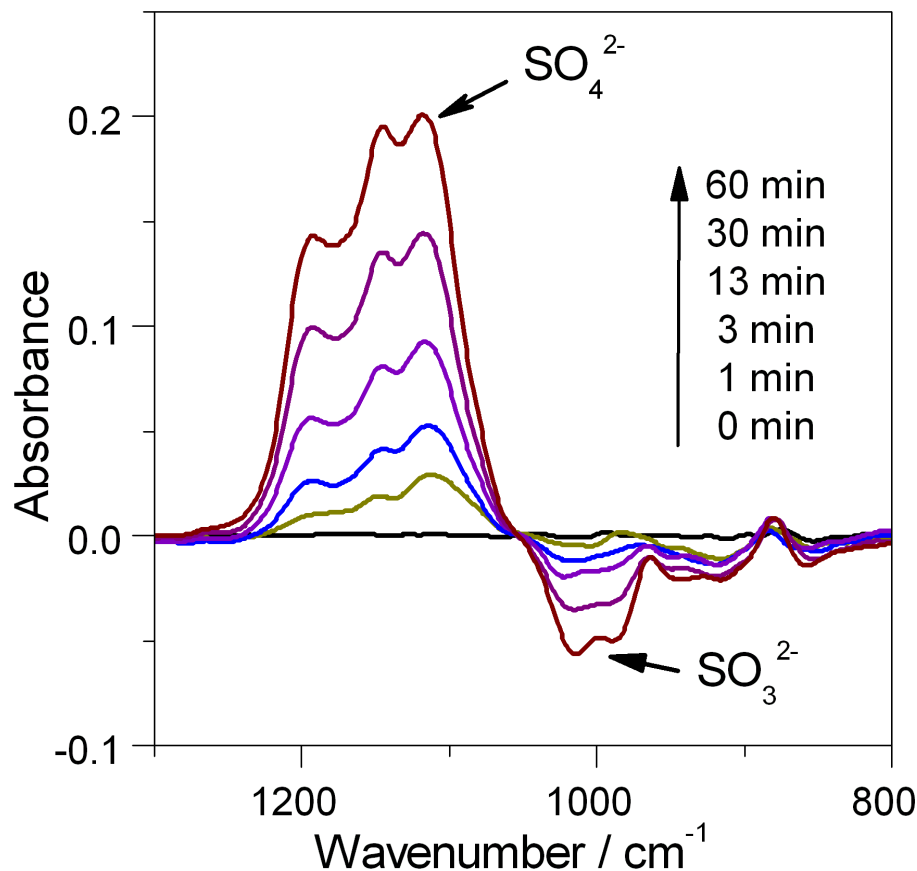
Fig. 3. In situ DRIFTS spectra of O 3 oxidation of sulfite mixed into CaCO 3 powder. The unexposed sample was used to collect a background spectrum and the sulfate positive band at 1100 cm -1 and the sulfite negative band at 1000 cm -1 changed with the reaction time.
