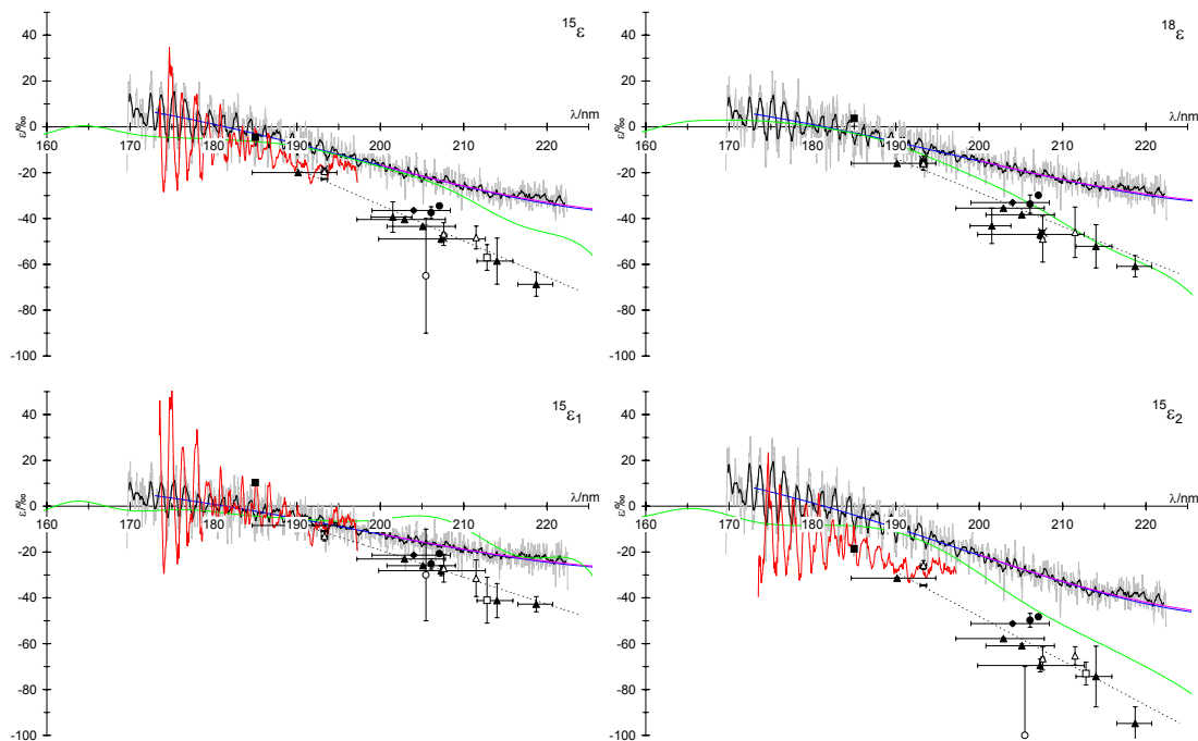
Fig. 3. Measured and theoretically predicted fractionation constants for \text{N}_2\text{O} photolysis at room temperature (unless indicated:) continued ....
