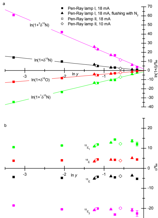
Fig. 1. Rayleigh fractionation plot (panel a ) of \ln(1 + \delta) vs \ln y and directly calculated fractionation constants \epsilon (panel b ) for photolysis with low-pressure Hg(Ar) lamps at 185 nm. y is the remaining N_2O fraction. Fractionation constants for the terminal and central nitrogen positions in the N_2O molecule are designated ^{15}\epsilon_1 and ^{15}\epsilon_2 ; the ^{18}O fractionation is represented by ^{18}\epsilon and the average ^{15}N fractionation by ^{15}\epsilon = (^{15}\epsilon_1 + ^{15}\epsilon_2)/2 . The corresponding \delta values are ^1\delta^{15}N , ^2\delta^{15}N , \delta^{18}O and \delta^{15}N . Two different lamps were used at operating currents of 10 and 18 mA, with or without nitrogen flushing. Errors from N_2O extraction and isotope analysis are smaller than the symbol size, unless indicated.
