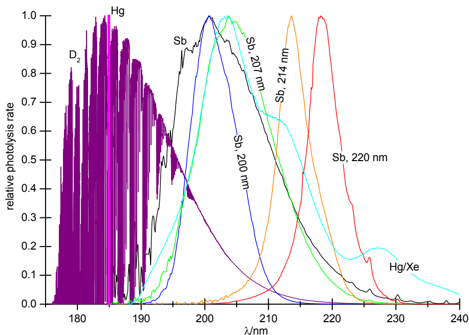
Fig. 2. Relative N 2 O photolysis rates for filtered and unfiltered light from different broadband lamps. The photolysis rates have been normalised by division through their maximum values so that they can be compared more easily. The closely spaced O 2 Schumann-Runge bands account for the structured appearance of the D 2 lamp spectrum.
