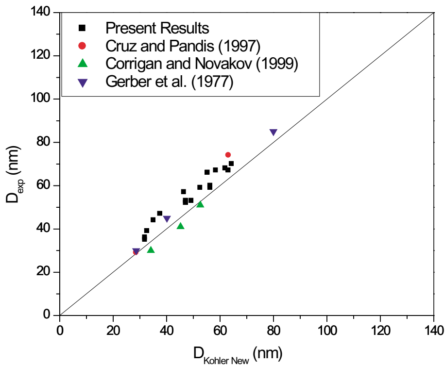
Fig. 6. Same plot as Fig. 5 except that the water activity in the Kohler prediction ( D_{\text{Kohler New}} ) has been taken from Clegg et al. (1996).
