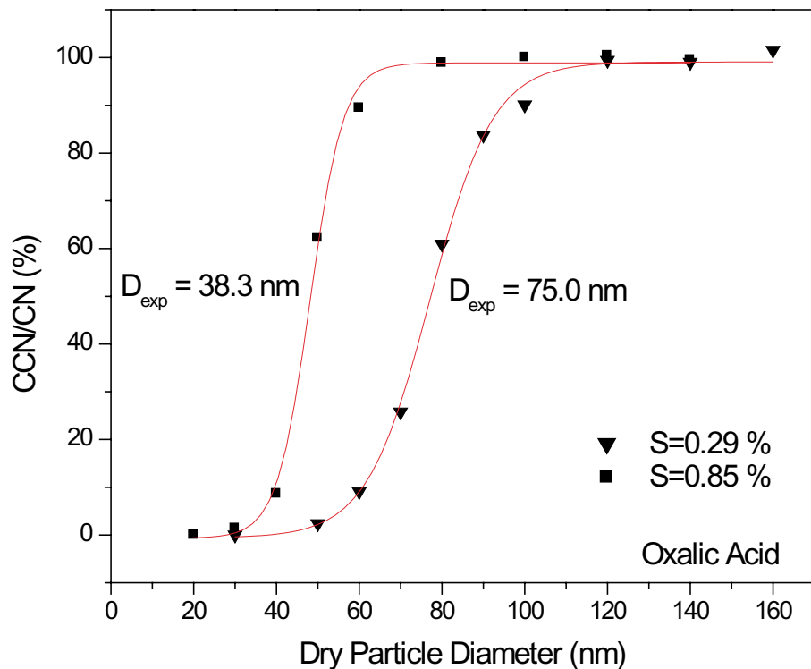
Fig. 7. Ratio of the number of activated droplets (“CCN”) relative to the number of condensation nuclei (“CN”) plotted as a function of dry particle diameter for oxalic acid particles at supersaturations of 0.29 and 0.85%. Vertical axis has been corrected to indicate full activation (see text for explanation).
