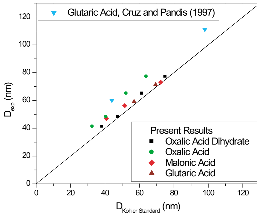
Fig. 9. For all organic acids studied in this work, comparison between the experimental values of the dry particle diameter that give 50% activation ( D_{\text{exp}} ) and the theoretical predications of this quantity from standard Kohler theory ( D_{\text{Kohler Standard}} ) described by Eqs. (1), (2) and (3). Each point represents an experiment conducted at a fixed supersaturation between 0.29 and 0.85%. Also included are results from the literature. For oxalic acid, two sets of points are included assuming formation of anhydrous oxalic acid and oxalic acid dihydrate, respectively.
