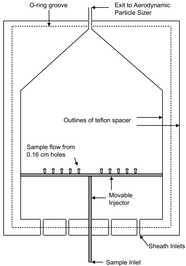
Fig. 2. Horizontal cross-section of the thermal-gradient diffusion chamber.
