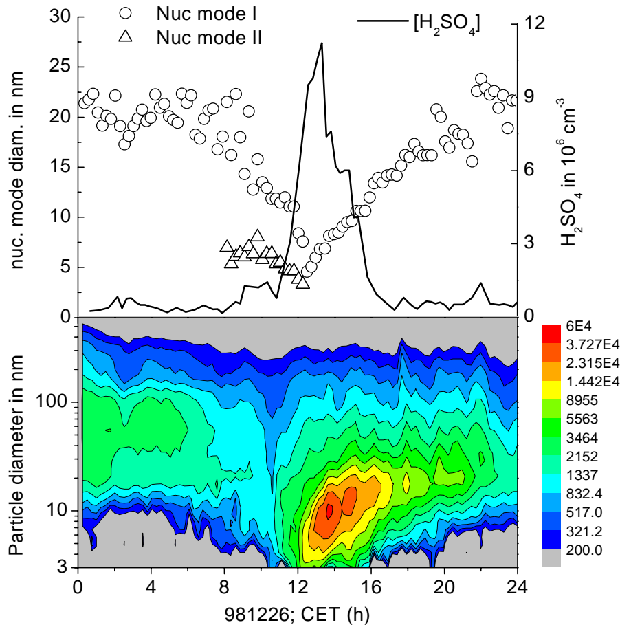
Fig. 13. Time series of the particle size distribution ( dN/d\log D_p in \text{cm}^{-3} ), the nucleation mode diameter, and H_2SO_4 . Data is from 26 December 1998, a winter class I event day.
