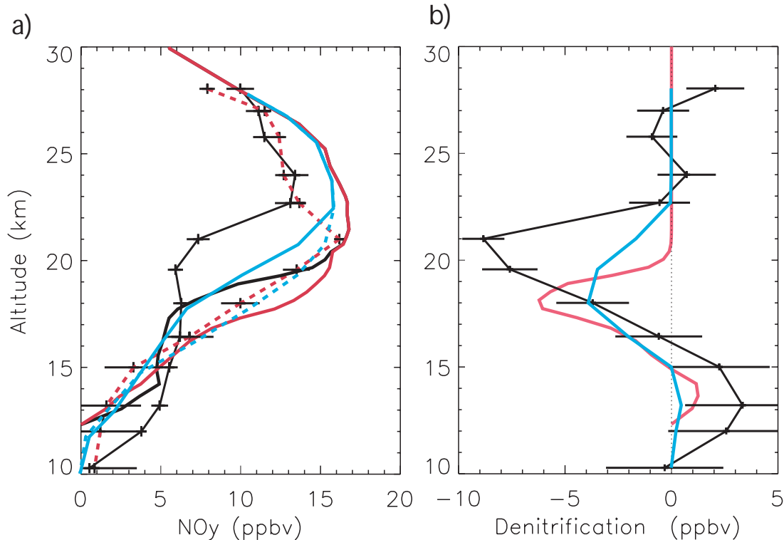
Fig. 13. (a) Comparison of MIPAS-B observed \text{NO}_y (black) and \text{NO}_y^* (dashed black) with DLAPSE/SLIMCAT \text{NO}_y and model passive \text{NO}_y on 25 February 1995. Pairs of (a) MIPAS-B \text{NO}_y (black), MIPAS-B \text{NO}_y^* (dashed black), model \text{NO}_y (red) and model passive \text{NO}_y (dashed red) shown. Blue lines indicate model degraded to 3 km vertical resolution; (b) Diagnosed denitrification from (a).
