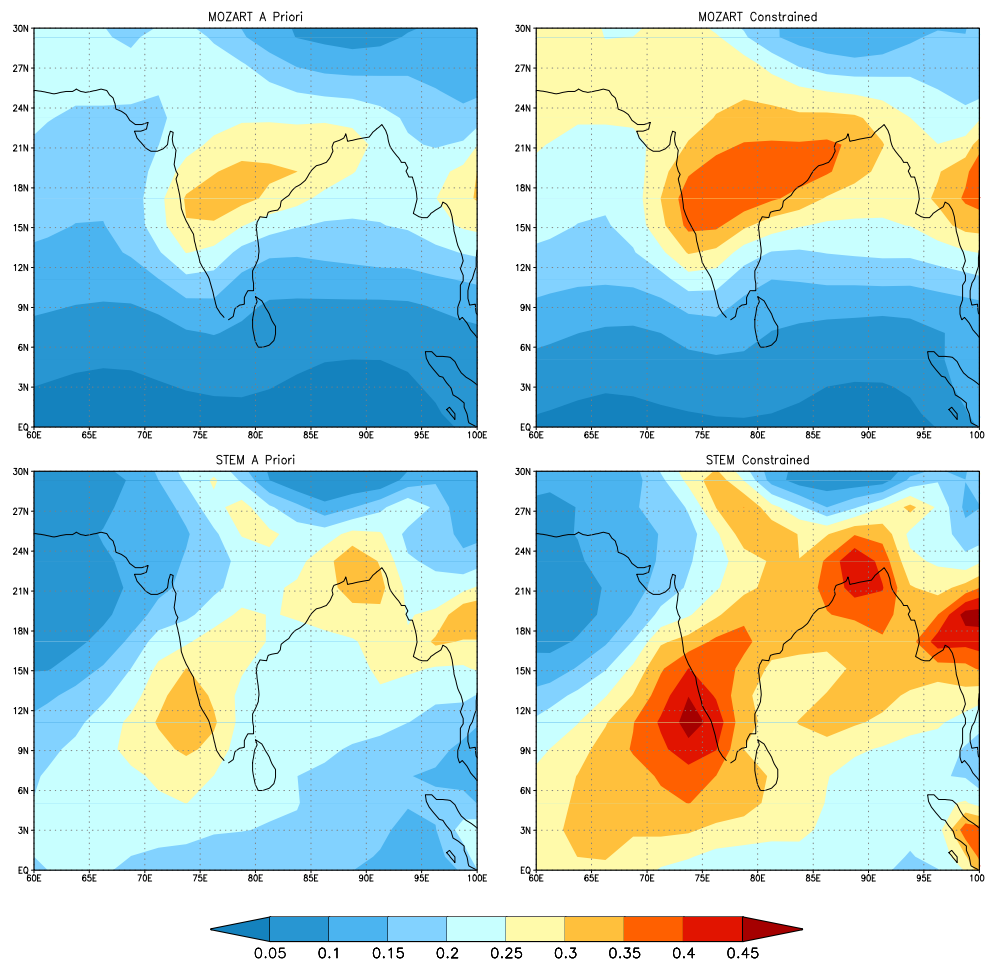
Fig. 18. NIO AOD at 0.55\ \mu\text{m} with MOZART aerosols (top panel) and STEM aerosols (bottom panel). First column is with the “a priori” aerosol optical properties; second column is with the constrained optical properties.
