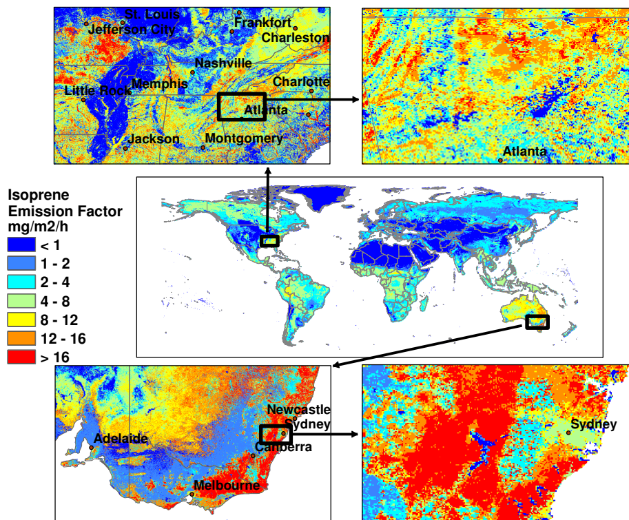
Fig. 9. Global distribution of landscape-average isoprene emission factors ( \text{mg} isoprene \text{m}^{-2} \text{h}^{-1} ). Spatial variability at the base resolution ( \sim 1 km) is shown by regional images of the southeastern U.S. and southeastern Australia.
