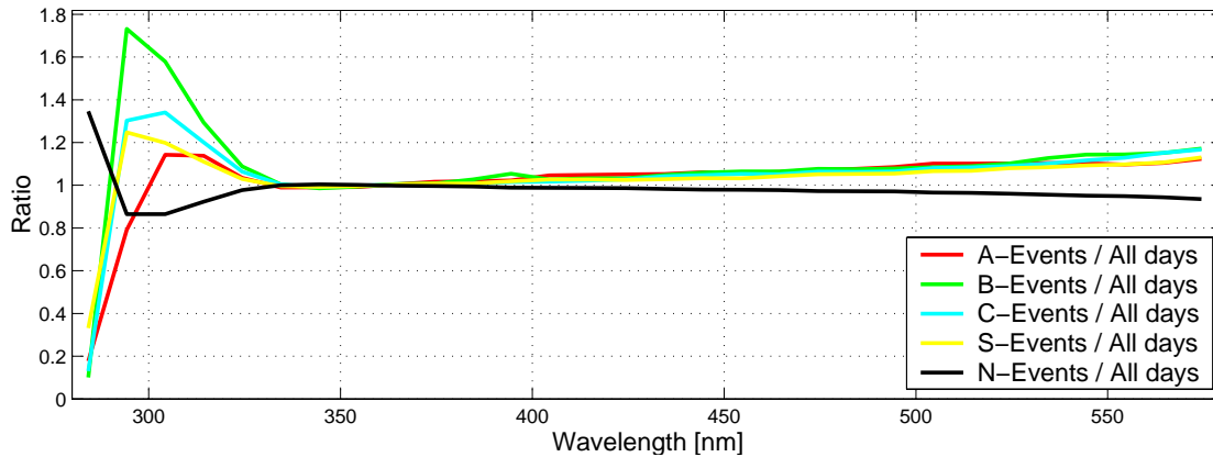
Fig. 5. (a) Average spectral solar irradiance for all event and non-event classes of 2000 and 2001; (b) Ratio of the graphs from (a) to a yearly reference graph from Eq. (4) ( \overline{E_{G,N}} ).
