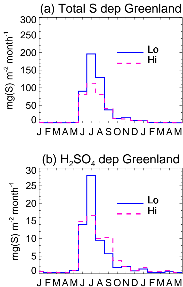
Fig. 9. Simulated monthly (a) total sulphur and (b) H 2 SO 4 deposition fluxes (mg(S) m -2 month -1 ) to central Greenland, for the two Laki scenarios.
