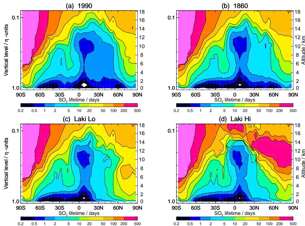
Fig. 2. Zonal, June-July-August (JJA) mean SO 2 lifetimes (days) for: (a) 1990; (b) 1860; (c) Laki Lo; and (d) Laki Hi.
