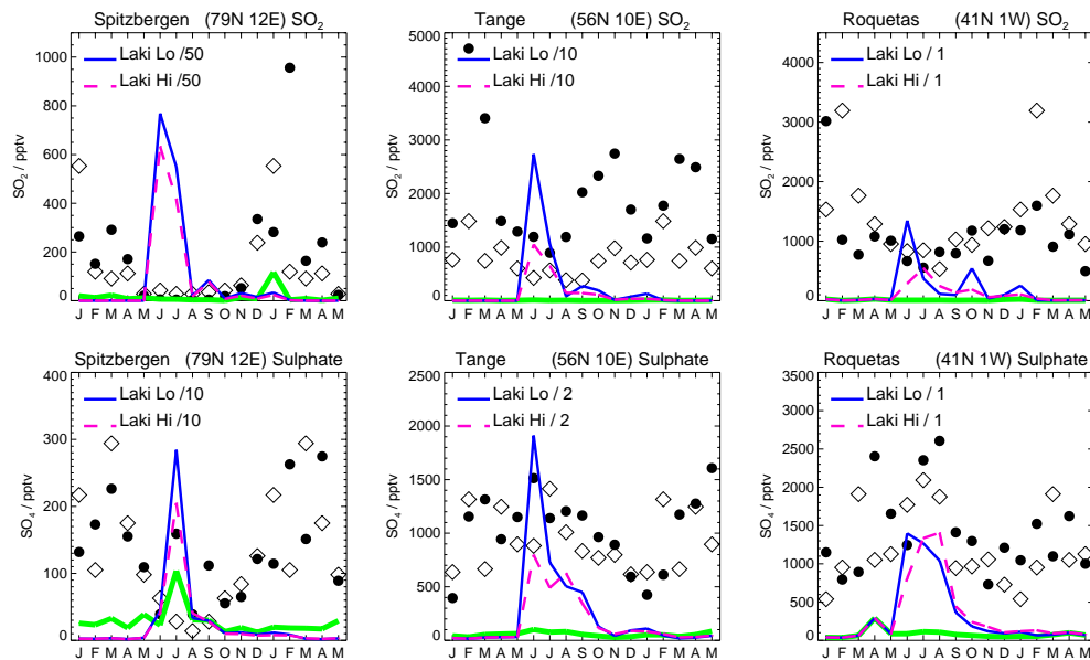
Fig. 6. Comparison of 1990 modelled \text{SO}_2 and \text{SO}_4 (•) with recent observations ( \diamond ) (Hjellbrekke et al., 1996) at 3 European sites. The plot extends over 17 months of model results; observations are repeated for the second year. Also shown are results from the 1860 scenario (thick green line), and the two Laki scenarios (solid blue and dashed magenta lines), reduced by up to a factor of 50 to fit on the plots.
