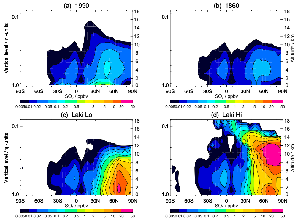
Fig. 1. Zonal, June-July-August (JJA) mean SO 2 concentrations (ppbv) for: (a) 1990; (b) 1860; (c) Laki Lo; and (d) Laki Hi.
