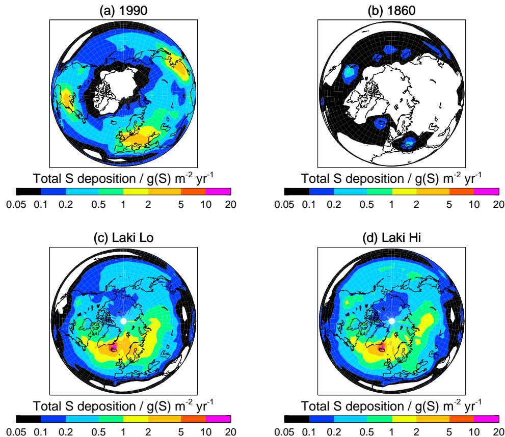
Fig. 8. Northern Hemisphere annual mean total sulphur deposition fluxes ( \text{g(S)} \text{ m}^{-2} \text{ yr}^{-1} ) for: (a) 1990; (b) 1860; (c) Laki Lo; and (d) Laki Hi.
