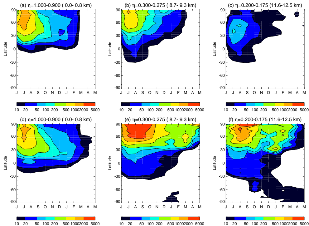
Fig. 7. Temporal evolution of the zonal mean Laki \text{SO}_4 (pptv) for Laki Lo ( a–c ) and Laki Hi ( d–f ), at three levels in the model: the surface ( a, d ); the upper troposphere ( b, e ); and the lower stratosphere ( c, f ). Background 1860 levels have been subtracted.
