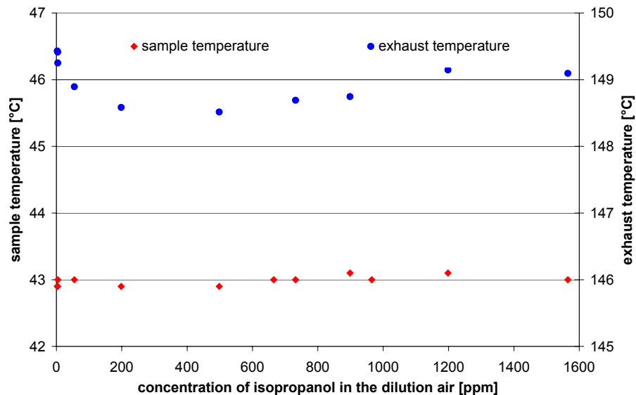
Fig. 2. Variation of sample and exhaust temperatures as a function of the 2-propanol concentration in the sample air.
