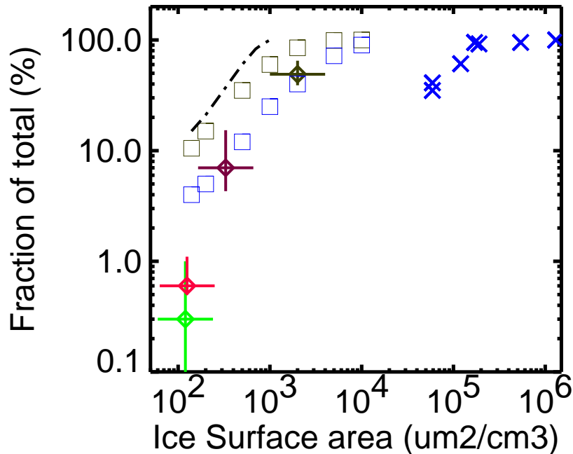
Fig. 3. HNO 3 partitioning in cirrus (in %) versus ice surface area; field and laboratory measurements (legend see Fig. 4) in comparison to the parameterization for low uptake of Lawrence and Crutzen (1998) (dashed dotted line) and model calculations of Tabazadeh et al. (1999) (open rectangles; blue: 230K, olive: 210K).
