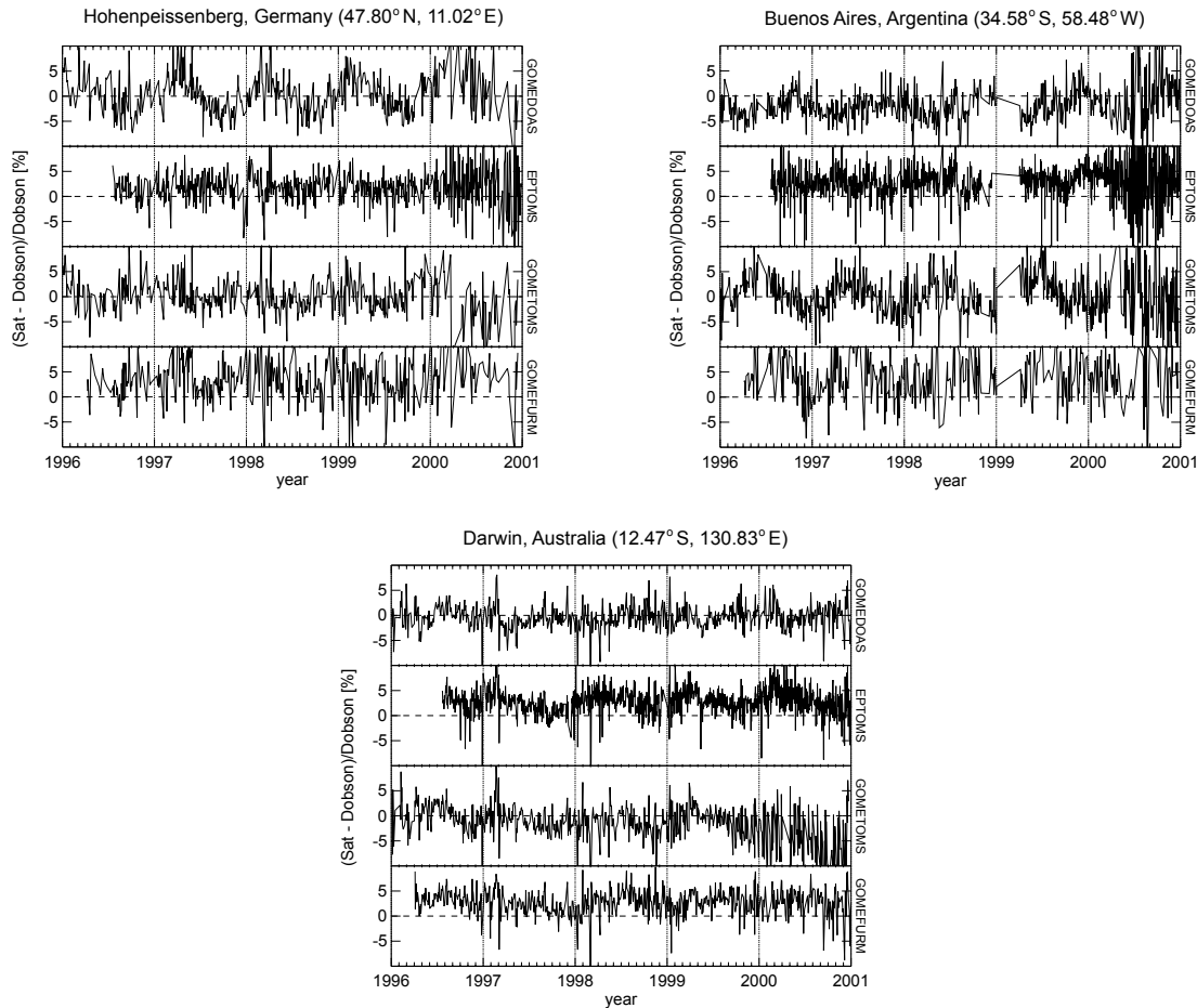
Fig. 3. Relative deviation between satellite and Dobson measurements for the stations Hohenpeissenberg, Buenos Aires, and Darwin.
