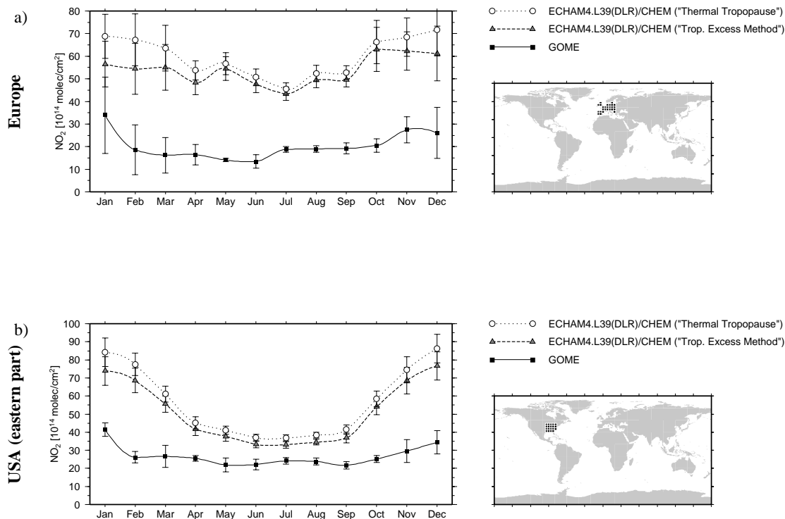
Fig. 4. (a – f): Seasonal variation of the tropospheric NO 2 column amounts for the climatological average values for selected spatial domains. The two sigma standard deviation of the individual monthly means to the climatological monthly means are drawn as errorbars for each data point. The small map to the right depicts the grid cells, that have been used to calculate the average values of the specified domain.
