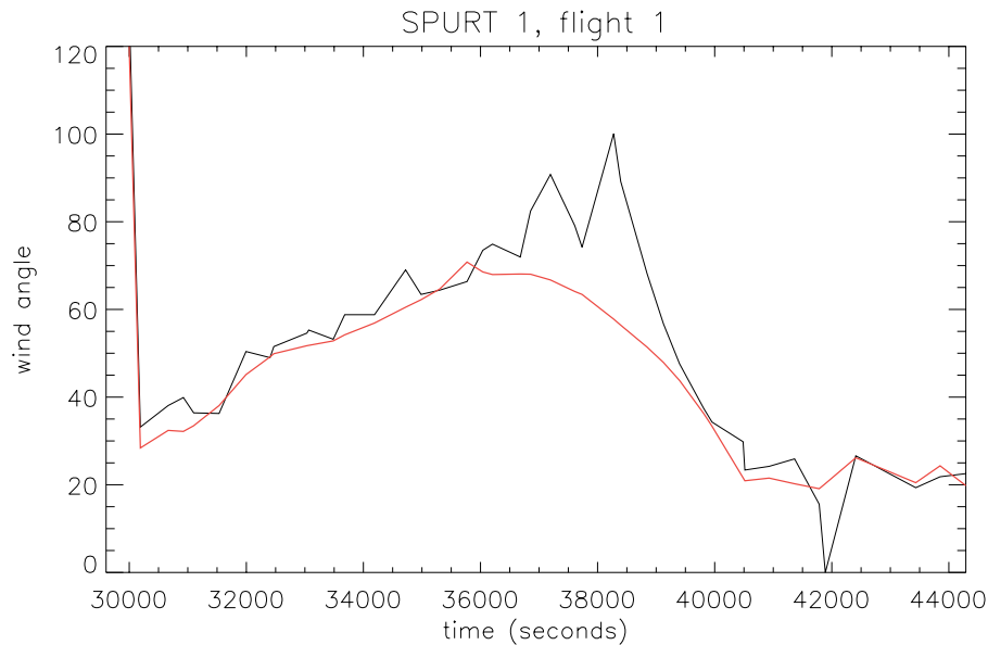
Fig. 11. By ECMWF analyzed wind along the flight path (red) and the wind measured by the aircraft instrumentation (black). The aircraft experienced wind with a more easterly component than given by the model, indicating that the flight path lied closer to the outflow region of the convective system over the western Mediterranean.
