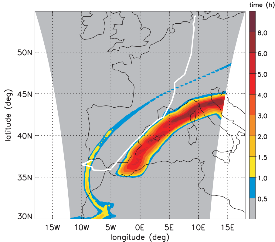
Fig. 9. Convective influence plot of the grid points on the 200 hPa level at 12:00 UTC. The color code indicates the total time (in h) during which the air parcels experienced higher temperatures than the underlying brightness temperature of the clouds during the previous 1.5 days, indicating that they passed through a cloud. The flight path is overlaid as white line.
