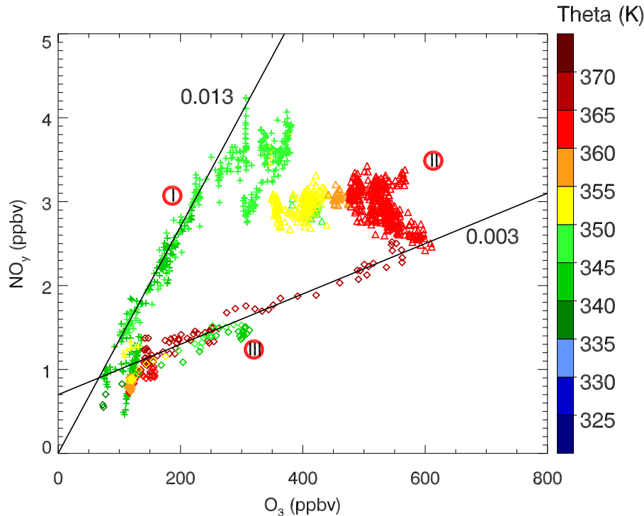
Fig. 3. Tracer correlation between O 3 and NO y as a function of potential temperature (color coded). In flight segment II (data points depicted as triangles) a strong deviation from the expected linear correlation can be seen. The slope of the correlation, d[\text{NO}_y]/d[\text{O}_3] = 0.003 , in flight segment III (diamonds) represents a typical value for air from the extratropical stratosphere. Flight segment I (crosses) includes data points with tropospheric mixing ratios of O 3 and NO y .
