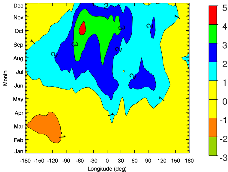
Fig. 4. 14-Year average seasonal cycle of \epsilon_2 as a function of longitude. A value of 1 denotes a difference of 5.3 DU ( 1-\sigma ) between model and observations. The +/- signs were added to the figure to signify model underestimates or overestimates respectively.
