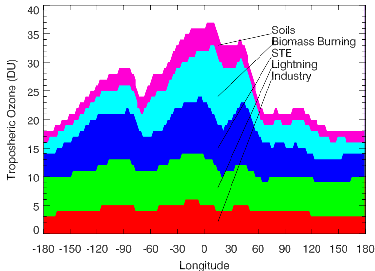
Fig. 6. Absolute contribution of several processes to the modeled TTOC distribution. Processes include photochemical production of ozone following \text{NO}_x emissions from soils, lightning, biomass burning and industrial sources, as well as ozone from stratosphere-troposphere exchange. Values for September 1992.
