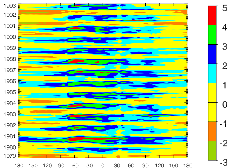
Fig. 3. Hövmoller plot of \epsilon_2 as a function of longitude for the period 1979–1992. A value of 1 denotes a difference of 5.3 DU ( 1-\sigma ) between model and observations. The +/- signs were added to the figure to signify model underestimates or overestimates respectively.
