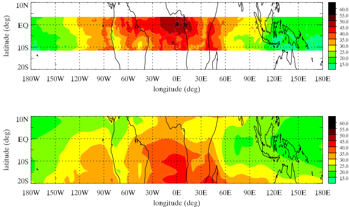
Fig. 1. Observed (top) and model calculated (bottom) distribution of TTOC in September 1992. Note the widespread underestimate of TTOC over the tropical Atlantic Ocean and adjacent continents.
