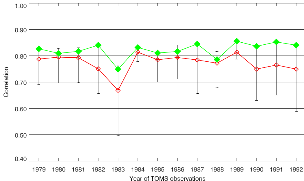
Fig. 5. Correlation coefficient ( \epsilon_1 ) between the zonal TTOC distribution in observations and simulations. For each year of TTOC observations (1979–1992) correlations were calculated with each year of a multi-year simulation with our CTM (1979–1992). The bars denote the range of correlations, the red diamonds are the averages. This value is representative for a simulation with ‘climatological’ meteorology. The green diamonds signify the correlation when the correct meteorology of the year of observations is applied to the model.
