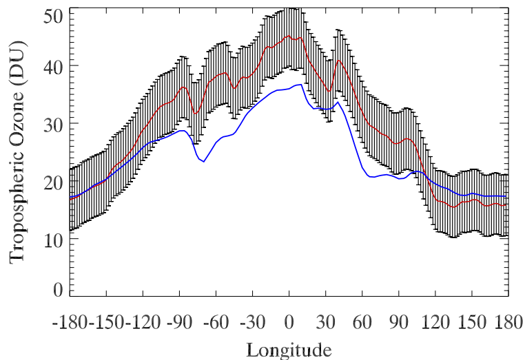
Fig. 2. The meridionally averaged zonal TTOC distribution in model calculated (blue) and satellite retrieved (red) TTOC for September 1992. This distribution is used to define a measure of error according to Eq. (1). The shaded lines denote one-sigma standard deviation (5.3 DU)
