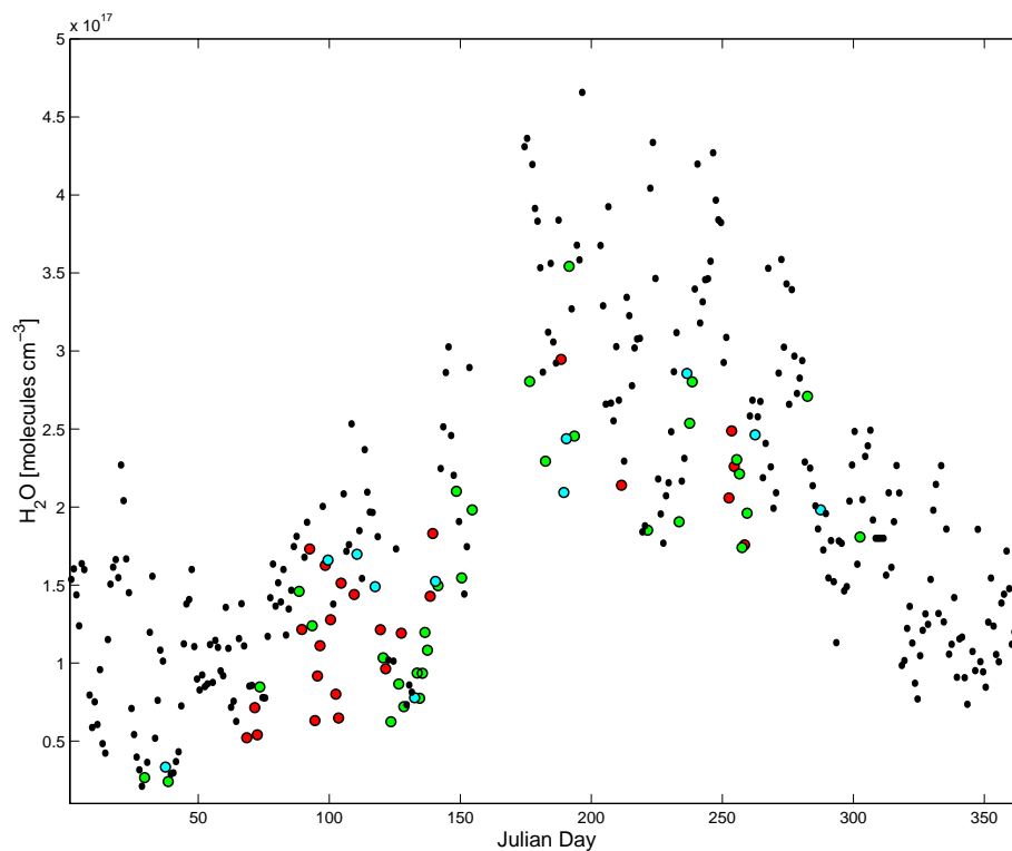
Fig. 7. Average values during the morning (9 to 11 a.m.) for the concentration of H 2 O at 67 m for the year 1999. A-, B- and C-Events are marked with red, green and cyan labels respectively and the non-event days are marked with black dots.
