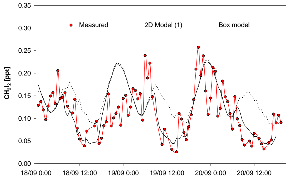
Fig. 9. Comparison of 2D model predictions of CH 2 I 2 , calculated using only coastal sources, with measurements and box model results.
