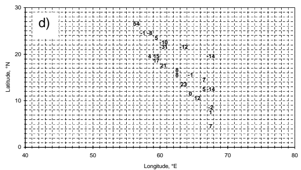
Fig. 5. Continued. Relative errors of the final field 1^\circ \times 1^\circ values. (a) DJF, (b) MAM, (c) JJA, and (d) SON.
