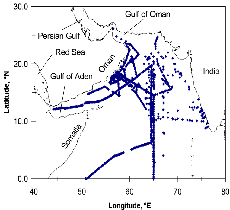
Fig. 1. Map of the Arabian Sea with locations of the \text{N}_2\text{O} measurements in the surface layer used in our study (see Table 1).
