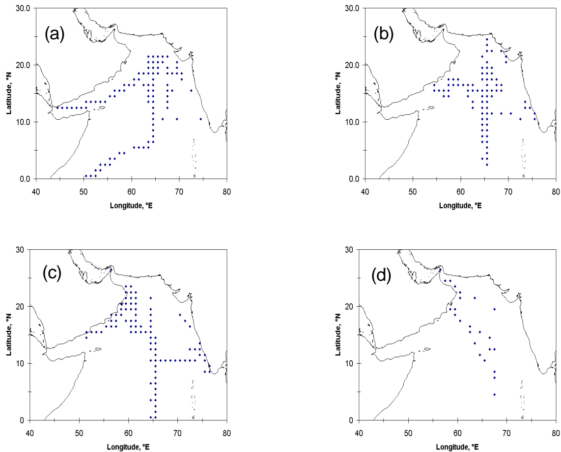
Fig. 2. Seasonal maps of N 2 O pixels. (a) DJF, (b) MAM, (c) JJA, and (d) SON.
