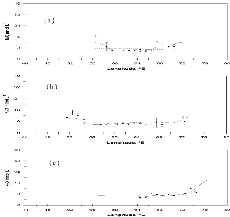
Fig. 4. Annual mean \text{N}_2\text{O} concentrations (in \text{nmol L}^{-1} ) along selected latitudes. The solid line is the predicted \text{N}_2\text{O} from the final 1^\circ \times 1^\circ field, the dashed line stands for the smoothed first-guess field, and the solid squares represent the annual mean \text{N}_2\text{O} with standard deviation of all measurements within the 1^\circ \times 1^\circ squares along the given latitude. (When less than 3 values were available no standard deviation is given.) (a) 18.5^\circ \text{N} , (b) 15.5^\circ \text{N} , and (c) 10.5^\circ \text{N} .
