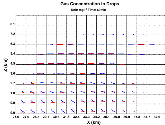
Fig. 10. As Fig. 9 but for H^* = 10^4 \text{ mol dm}^{-3} \text{ atm}^{-1} .
