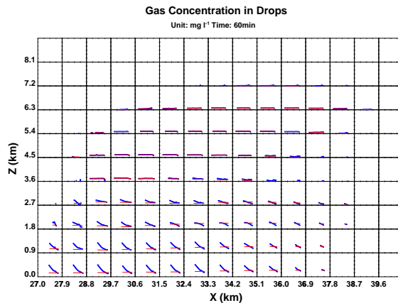
Fig. 10. As Fig. 9 but for H^* = 10^4 \text{ mol dm}^{-3} \text{ atm}^{-1} .
