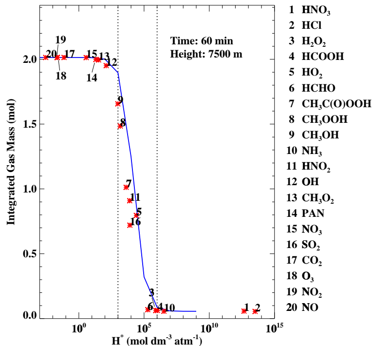
Fig. 13. The effect of the temperature dependence of the Henry's law constant on the gas abundance at 7500 m altitude. The line shows the maritime-sheared simulation (with constant H^* ) and the symbols are results for the 20 real gases listed on the right (for p\text{H}=5 ). Note that these simulations do not account for any chemical reactions that these gases may undergo in the liquid or gas phase and are meant to illustrate only the sensitivity to the temperature dependence of solubility.
