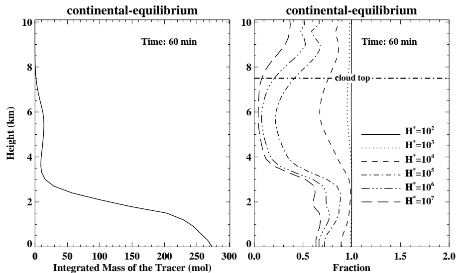
Fig. 12. Similar to Fig. 8 but for the continental-equilibrium simulation in which the gases and droplets are assumed to be in Henry's law equilibrium.
