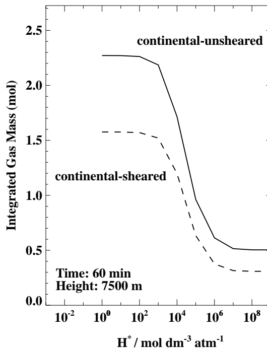
Fig. 7. A comparison of the integrated total species abundance as a function of effective Henry's law constant at 7500 m altitude (just below cloud top) for the continental-unsheared cloud (solid line) and the continental-sheared cloud (dashed line) after 60 mins of simulation. The width of the cloud in the y direction was normalized to 1 km to calculate the integrated gas mass).
