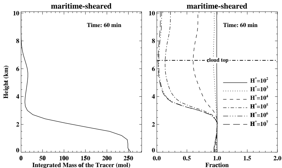
Fig. 8. (a) Vertical profile of the integrated total abundance of the insoluble tracer in the maritime-sheared simulation; (b) the abundance of soluble gases normalized to the abundance of the tracer.
