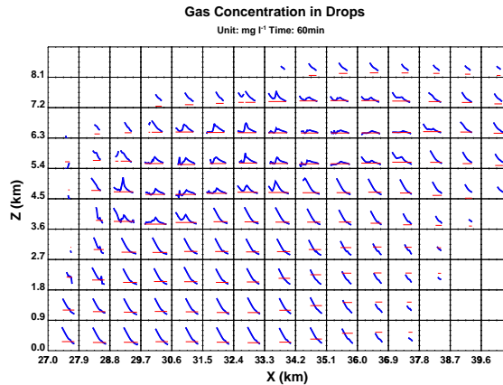
Fig. 11. As Fig. 9 but for H^* = 10^6 \text{ mol dm}^{-3} \text{ atm}^{-1} .
