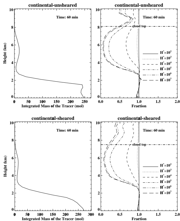
Fig. 6. Vertical profiles of the integrated species mass (gas phase + dissolved) as a fraction of that of the insoluble tracer for the continental-unsheared (top panels) and the continental-sheared (bottom panels) clouds after 60 min of simulation. The cloud top ( q_c > 10^{-3} \text{ g kg}^{-1} ) is also indicated.
