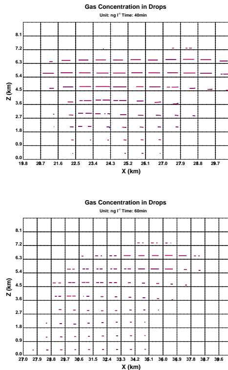
Fig. 9. Distributions of dissolved gas concentration inside drops at different locations after 40 and 60 min of simulation for the continental-sheared (blue lines) and continental-equilibrium (red lines) simulations. The solubility of the gas is equal to 10^2 \text{ mol dm}^{-3} \text{ atm}^{-1} . In one box the tick values for the abscissa are 1, 10, 1000, and 10000 \mu\text{m} , and the range for the ordinate values are from 10^{-2} to 10^4 . It should be noted that the unit in this figure is different from Fig. 10 and 11.
