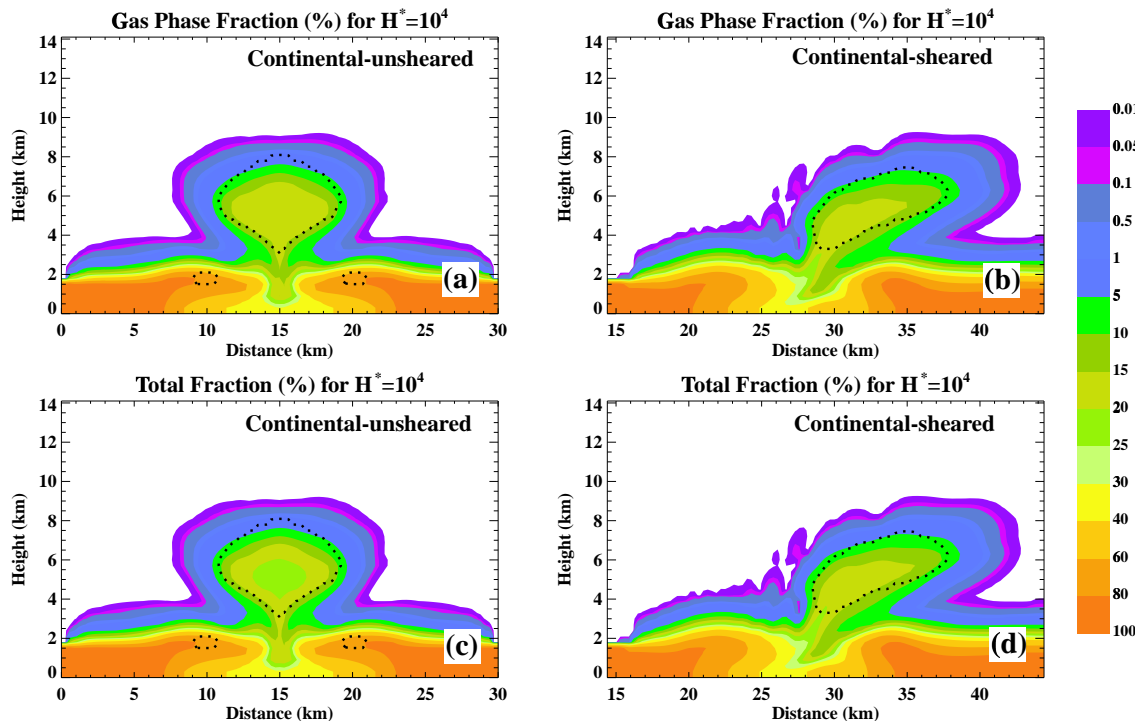
Fig. 4. Spatial distributions after 60 minutes of simulation of the mixing ratio of a moderately soluble gas ( H^* = 10^4 mol dm -3 atm -1 ) as a fraction (percent) of the initial boundary layer value for (a) the gas-phase abundance in the continental-unsheared case, (b) the gas-phase abundance in the continental-sheared case, (c) the total abundance (gas-phase plus liquid-phase) in the continental-unsheared case, and (d) the total abundance in the continental-sheared case. The area within the black dotted line indicates visible cloud ( q_c > 10^{-3} g kg -1 ).
