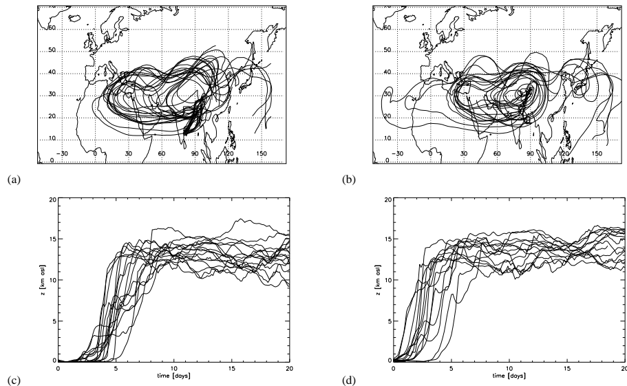
Fig. 5. 20-day forward trajectories for two big Indian cities (a) Madras ( 80.76^\circ E/ 13.85^\circ N, SE India) and (b) Patna ( 85.72^\circ E/ 26.01^\circ N, NE India) in July, 2001. Figure 5c shows the temporal development of the trajectory height above sea level for the (c) Madras trajectories and (d) for those from Patna.
