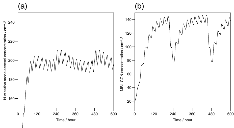
Fig. 4. Predicted variations in (a) nucleation and (b) accumulation mode aerosols. The entrainment terms were included in this case. The averaged concentration for N_1 and N_2 were 198 and 126 cm -3 , respectively.
