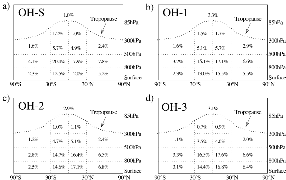
Fig. 4. The percentages of CH 4 which are oxidized in various subdomains of the atmosphere based on four different OH distributions: (a) OH-S; (b) OH-1; (c) OH-2; (d) OH-3.
