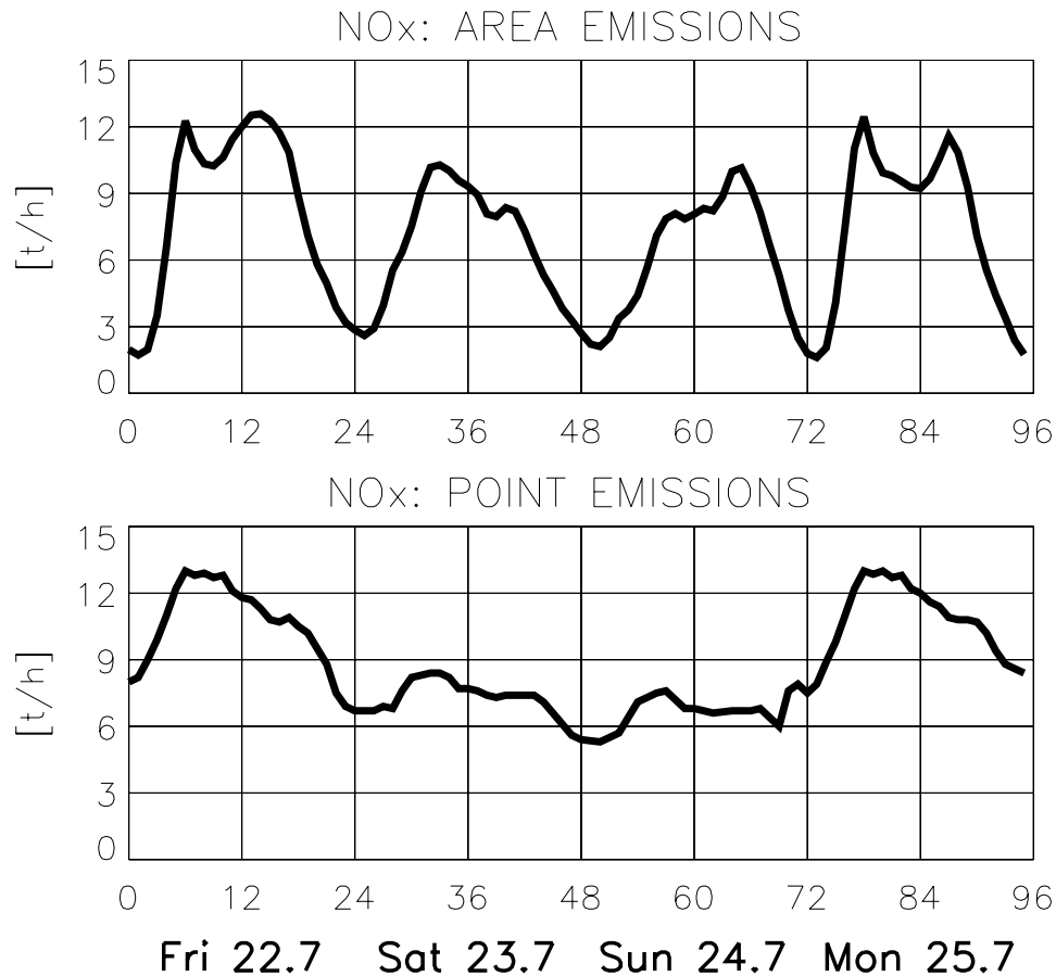
Fig. 4. Time series of NO x emission as sum of all area emission sources (upper panel) and point sources (lower panel) released into the domain between 22 and 25 July. The emissions are in units of [t/h].
