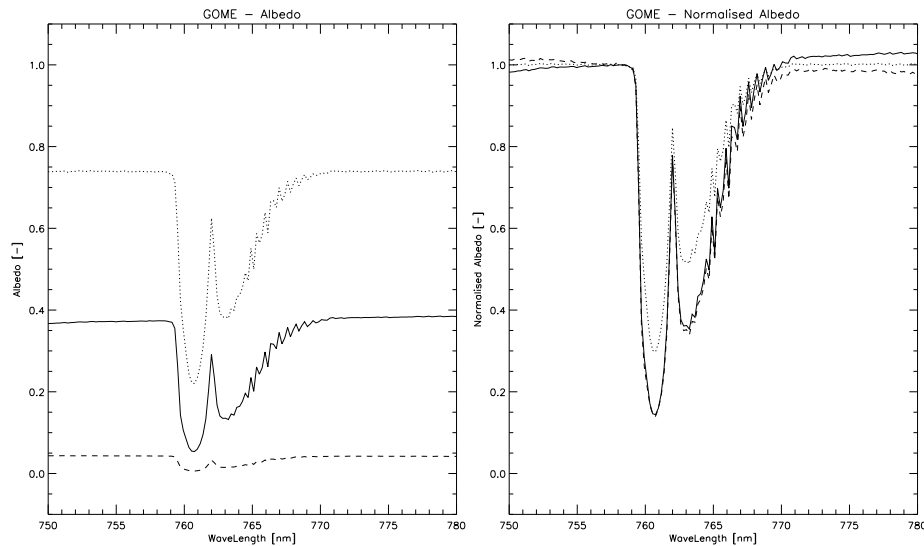
Fig. 3. Left: Reflectance measured by GOME near the O 2 -A absorption band. The dotted line is a fully cloudy scene, the solid line is a clear sky situation over land (the Netherlands), the dashed line is a clear sky situation over sea (the Atlantic Ocean). Right: Normalised albedo of the same situations (normalization wavelength \lambda_n = 758.0 nm).
