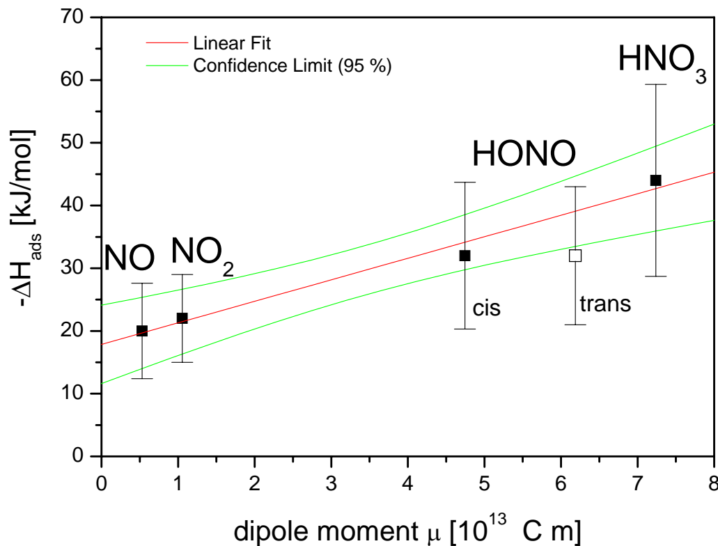
Fig. 5. Correlation of dipole moment (Lide, 2001–2002) and the experimentally found adsorption enthalpy for \text{NO} , \text{NO}_2 and \text{HNO}_3 .
