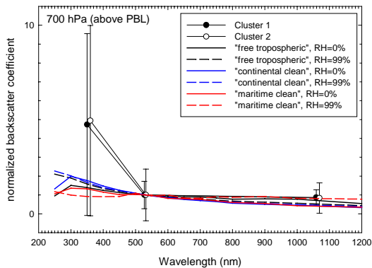
Fig. 13. Mean backscatter coefficients measured in the individual clusters given in Fig. 11, normalized to the value measured at 532 nm. Upper panel: in PBL, lower panel: above PBL. The error bars indicate the standard deviation inside the clusters. For clarity, an offset of 10 nm was added to wavelengths, centered around the real value. Also shown are selected aerosol types from the Global Aerosol Data Set (GADS).
