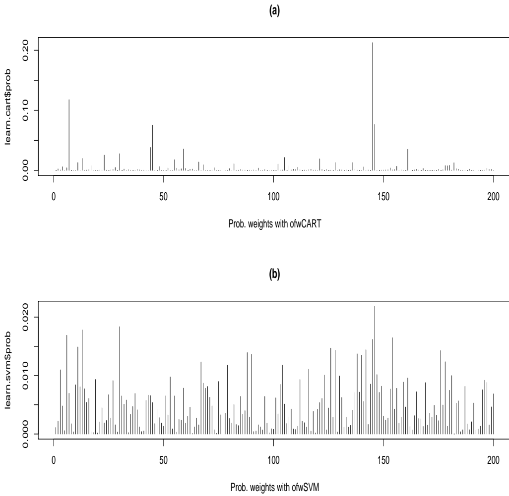
Figure 3: Probability weights with ofwCART (a) and ofwSVM (b).
