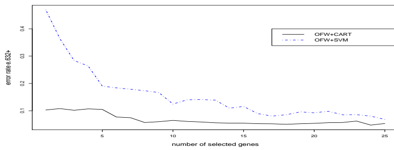
Figure 4: e.632+ error rate of ofwCART and ofwSVM.
