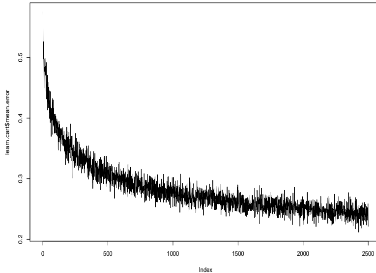
Figure 2: Internal mean error in ofwCART.
