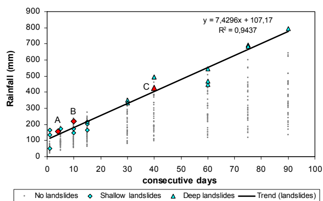
Fig. 10. Regression line between critical cumulative rainfall amount and corresponding rainfall event duration. Diamonds: values associated to shallow landslide events; Triangles: values associated to deep landslide events; Small grey dots: values obtained from the yearly cumulative rainfall values, and maximum rainfall intensity for all duration intervals (computed for years without reported landslides). Landslide events occurred in 2006 are marked in red: A – 20 March 2006; B – 27 October 2006; C – 28 November 2006.
