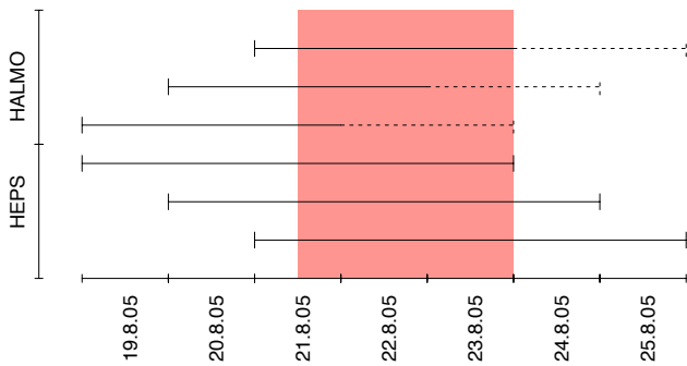
Fig. 3. Defined event period (red, 21 August 2005 12:00 UTC – 23 August 2005 24:00 UTC) with overlapping simulation ranges. The bars indicate the forecast periods of the ensembles (HEPS, 120 h) and the deterministic run (HALMO, 72 h). The dashed lines indicate the extension of the deterministic simulations to 120 h (see text for details).
