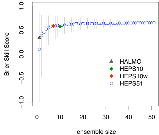
Fig. 7. Median BSS for sampled ensembles from HEPS51 with gradually reduced ensemble sizes, shown for catchment C10 (blue, with 90% quantile). BSS for HEPS10w (red, marked at effective ensemble size), HEPS10 (green) and HALMO (black) are additionally marked.
