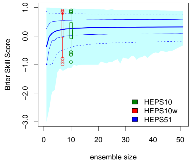
Fig. 8. Combined BSS for 23 subcatchments and three lead times as a function of ensemble size. The plot shows the median (bold blue line), the IQR (thin blue lines), the 90% quantile (dashed blue line) and the full range (light blue). The overlaid whisker plots show the BSS for HEPS10 (green) and HEPS10w (red).
