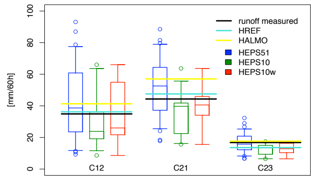
Fig. 6. Event discharges (mm/60h) for observed runoff (black), HREF (turquoise), HALMO (yellow), and whisker plots for the ensemble forecasts HEPS51 (blue), HEPS10 (green) and HEPS10w (red). Results are presented for the two catchments previously shown in Fig. 4 (C12, C21) and the catchment C23, representing the whole study area. All displayed forecasts are started on 20 August.
