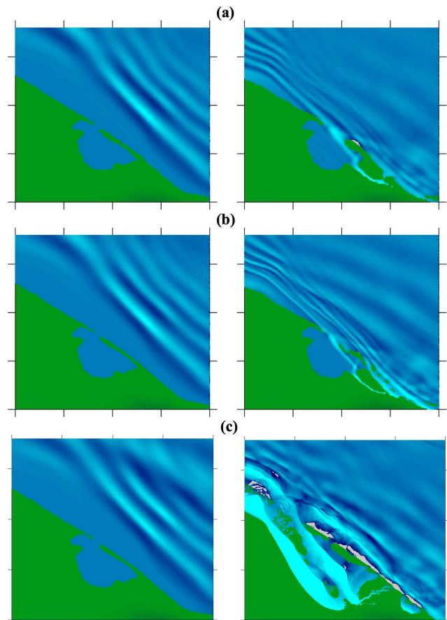
Fig. 9. A sensitivity analysis of our new Boussinesq simulation with respect to grid spacing. Snapshots of the free surface are shown at 18.8 min (left) and 23.8 min (right) after the main shock for: (a) uniform 200 \times 200 m grid spacing, (b) uniform 100 \times 100 m grid spacing, and (c) uniform 50 \times 50 m grid spacing. See text for further discussion.
