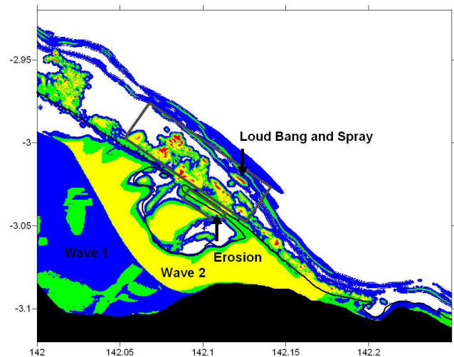
Fig. 7. Results from our new Boussinesq simulation carried out with a uniform 50 \times 50 m grid spacing. Map of maximum eddy viscosity v (as defined in FUNWAVE) localized on the front face of breaking waves: blue [very mild, v=0.01 ], green [mild, v=1 ], yellow [strong, v=9 ], red [very strong, v=40 ]. Regions of strongly nonlinear breaking waves and bores (yellow and red) are seen both offshore and onshore. A complex pattern occurs onshore from three different incident waves. See text for further discussion.
