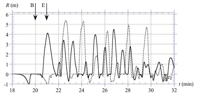
Fig. 8. Numerical tide gauges located in shallow water next to the villages of Malol (solid line), and Aitape (dashed line). The time of tsunami arrival relative to the aftershocks (B for “beginning” and E for “end” between 20 and 21 min after the earthquake) is correct at Malol although two minutes early at Aitape, because of the location of the numerical tide gauge relative to the village.
