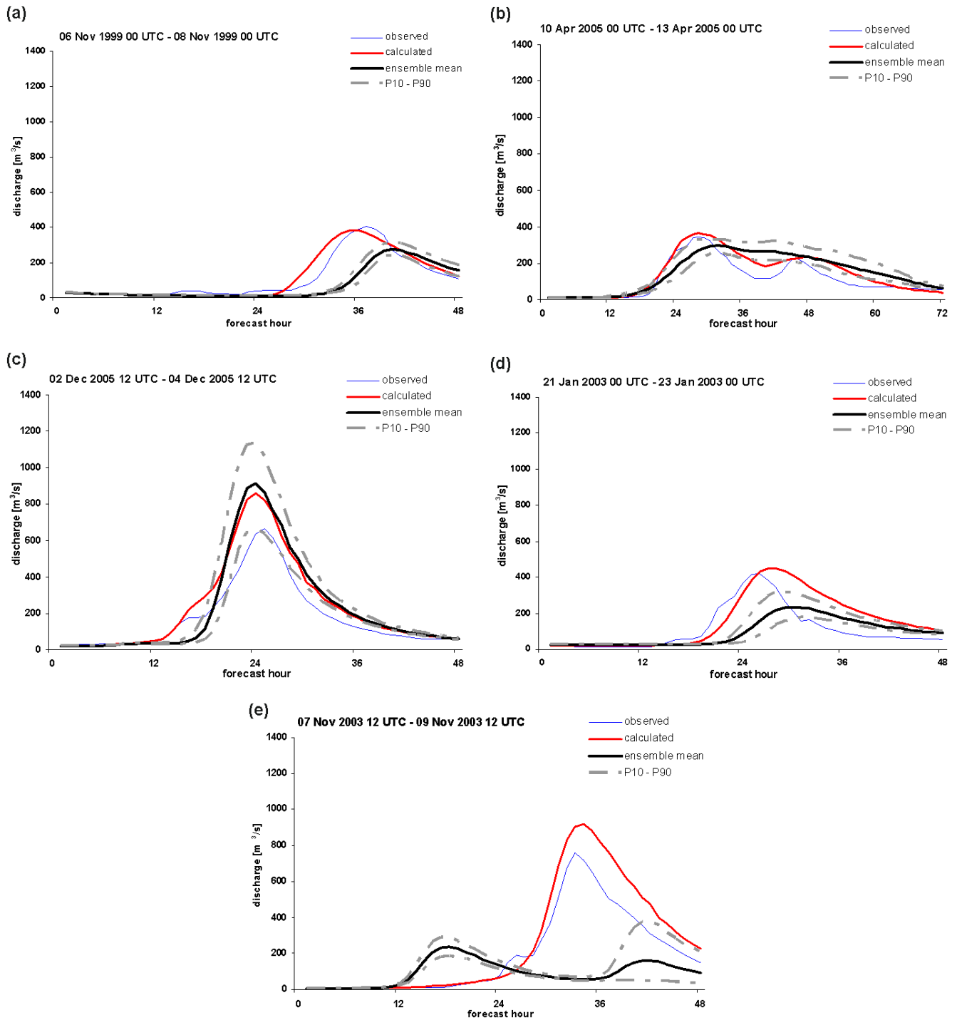
Fig. 12. Ensemble discharge forecasts (m 3 /s) vs. forecast time (h) for: (a) 6–7 Nov 1999 event; (b) 10–12 April 2005 event; (c) 2–3 Dec 2005 event; (d) 21–23 Jan 2003 event; (e) 7–9 Nov 2003 event. The bold line represents the ensemble mean, while the two grey dashed lines represent the P10 and P90 curves (see text). Red line is the discharge computed with rain gauge observation, blue line is the observed discharge.
